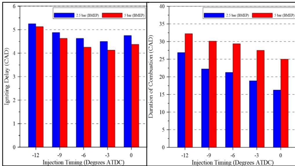
Figure ( 11) Ignition delay under high and low load
