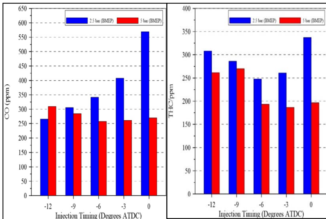
Figure ( 18 ) Effect of injection timing on carbon monoxide emissions under high and low load
