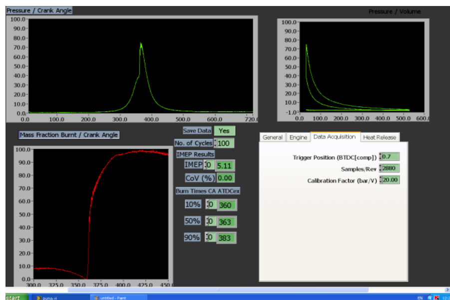
Figure (2) LabVIEW program screen
