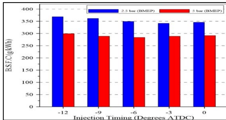
Figure ( 15 ) Effect of injection timing on The Brake Specific Fuel on sumpion (BSFC) under high and low load
