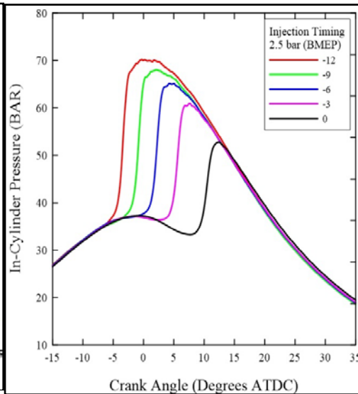
Figure.(6) In-cylinder pressure under 40Nm
