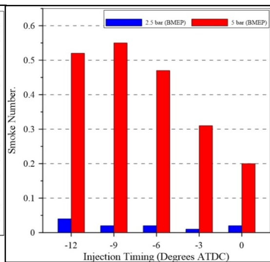
Figure ( 17 ) Effect of injection timing on smoke number under high and low load
