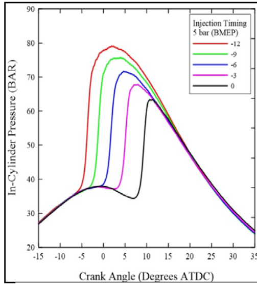
Figure.(5) In-cylinder pressure under 80Nm
