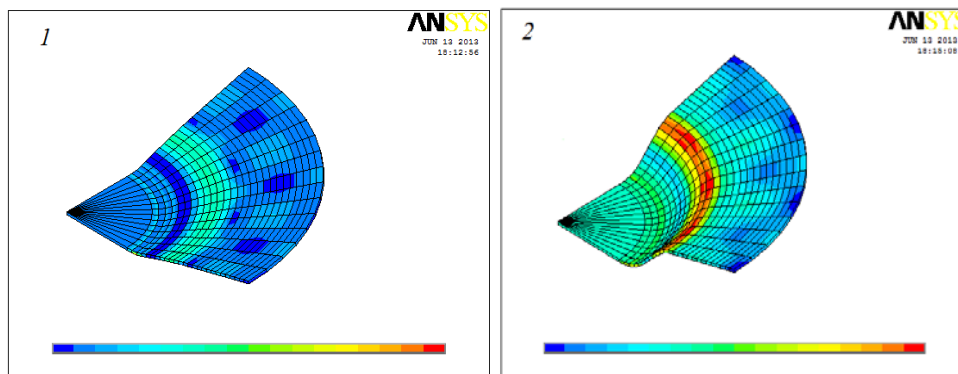
Figure (6) Deformation steps with sloping type BH.
