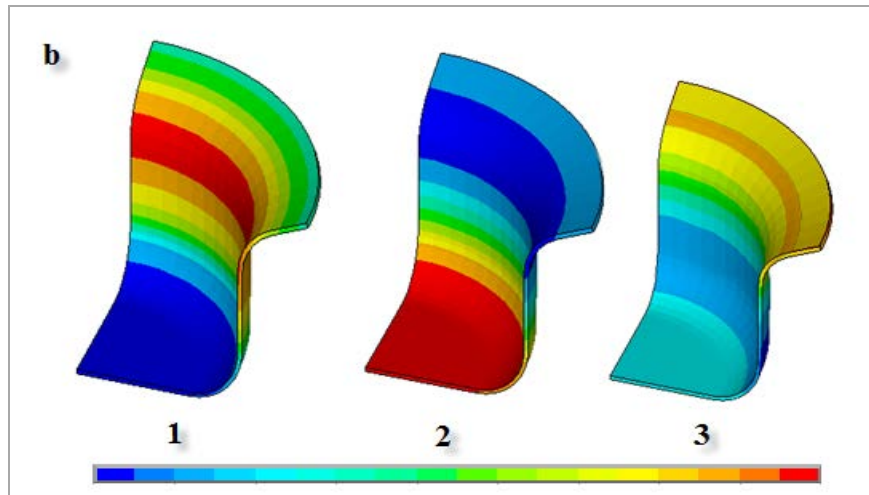
Figure (9) The strain distribution on the successful drawn cup (a-Flat model \alpha=0^\circ ) (b-Sloping model \alpha=22.5^\circ ) for 1- Radial strain.2-Hoop strain 3- Thickness strain.
