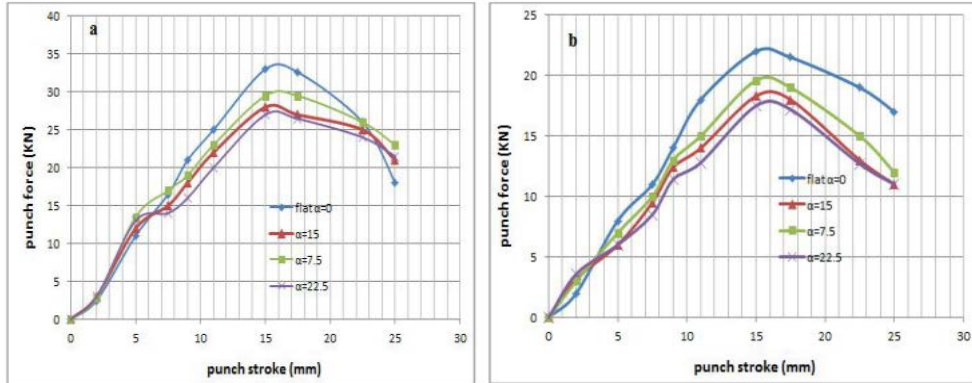
Figure (7) Effect of blank holder slope ( \alpha ) angle on punch force (a- experimental, b-FEA).
