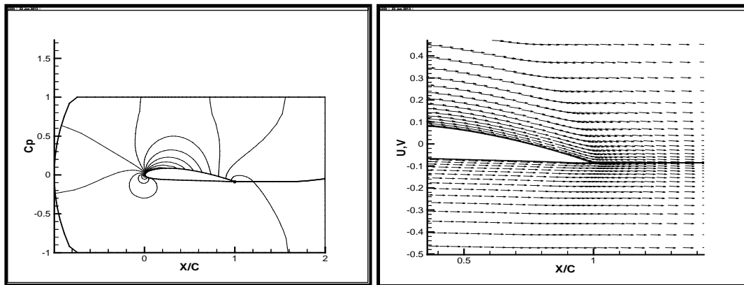
(b) Figure (13) Pressure distribution and flow stream of NACA 4415 at chord = 1.0, \alpha = 5^\circ, U = 5.0 (a) without blowing. (b) with blowing (at \alpha_{blowing} = -10^\circ and U_{blowing} = 10 )
