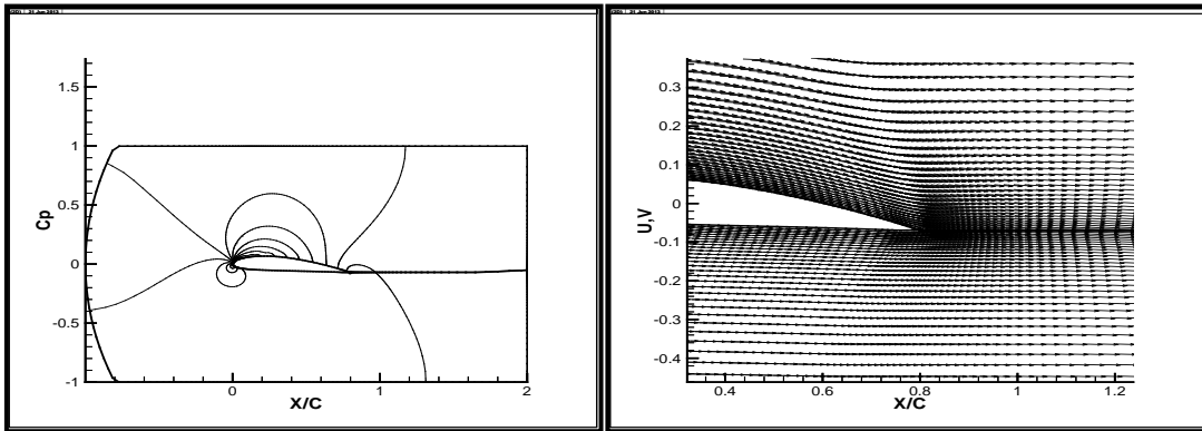
(b) Figure (7) Pressure distribution and flow stream of NACA 4415 at chord = 0.8, \alpha = 5^\circ , U = 5.0 (a) without blowing. (b) with blowing (at \alpha_{blowing} = -10^\circ and U_{blowing} = 10 )
