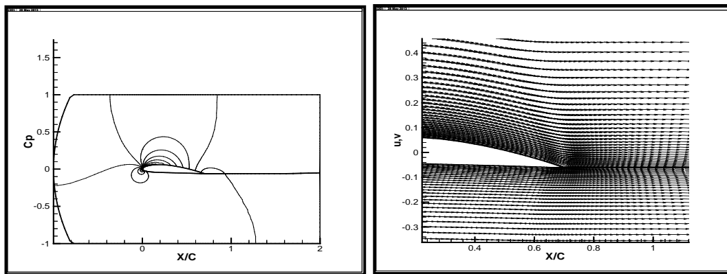
(a) (b) Figure (2) Pressure distribution and flow stream of NACA 4415 at chord = 0.6, \alpha = 10^\circ, U = 5.0 (a) without blowing. (b) with blowing (at \alpha_{blowing} = -10^\circ and U_{blowing} = 10 )
