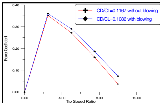
(a) NACA 4415 at chord 1.0
