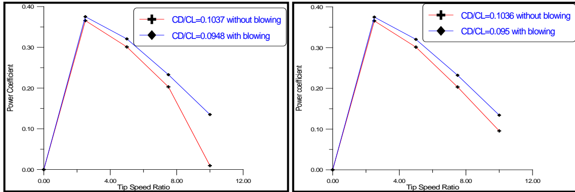
(c) NACA 4415 at chord 0.8
