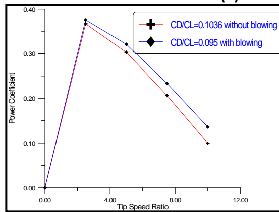
(e) NACA 4415 at chord 0.6
