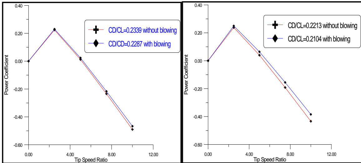
(c) NACA 4415 at chord 0.8
