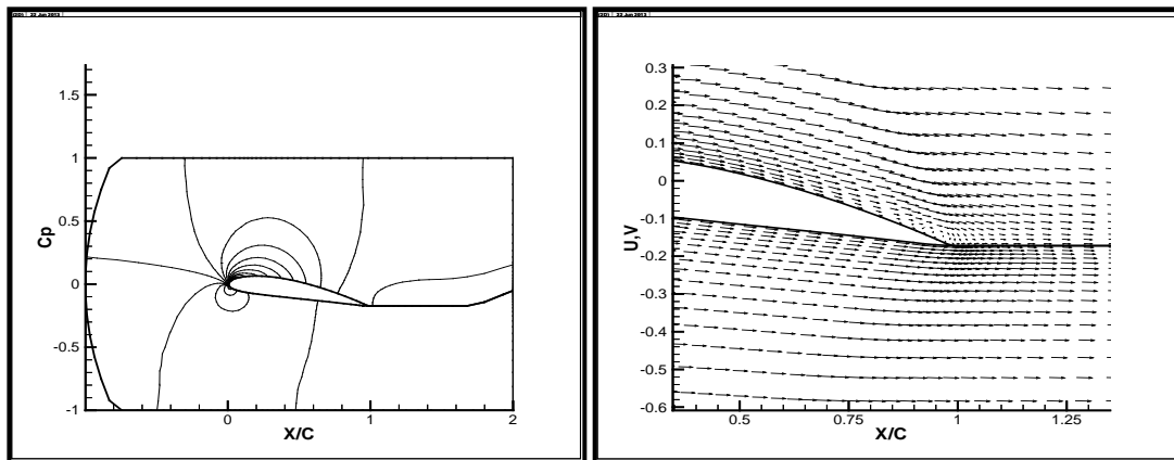
(a) (b) Figure (14) Pressure distribution and flow stream of NACA 4415 at chord = 1.0, \alpha = 10^\circ, U = 5.0 (a) without blowing. (b) with blowing (at \alpha_{blowing} = -10^\circ and U_{blowing} = 10 )
