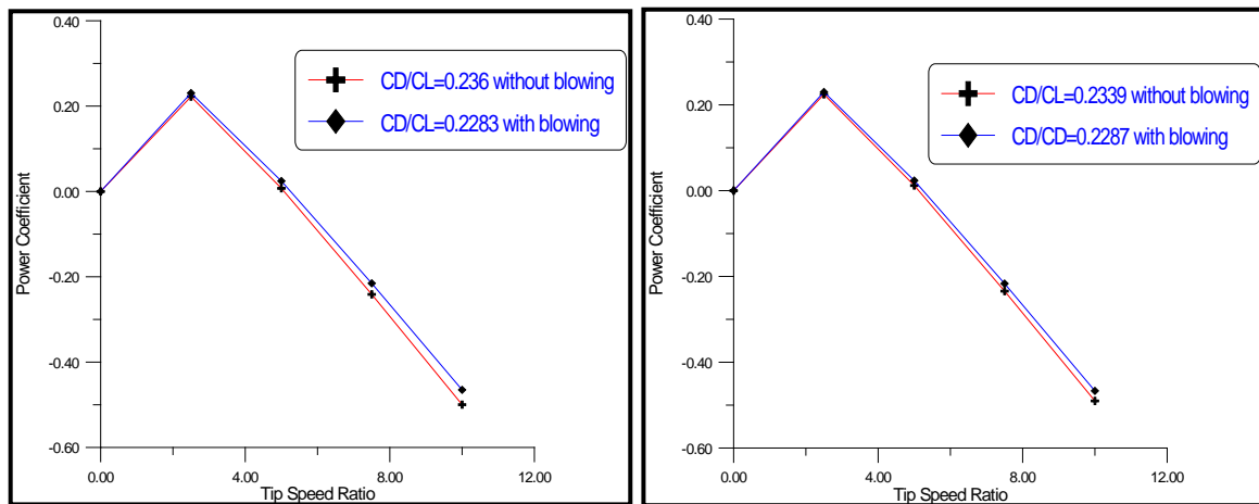
(a) NACA 4415 at chord 1.0
