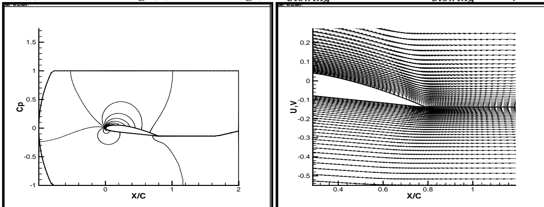
(a) Figure (8) Pressure distribution and flow stream of NACA 4415 at chord = 0.8, \alpha = 10^\circ , U = 5.0 (a) without blowing. (b) with blowing (at \alpha_{blowing} = -10^\circ and U_{blowing} = 10 )
