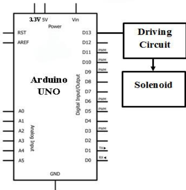
Fig. 11. Solenoid valve interfacing.
