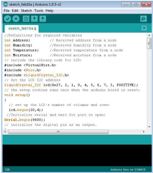
Fig.16 The Arduino software screenshot.
