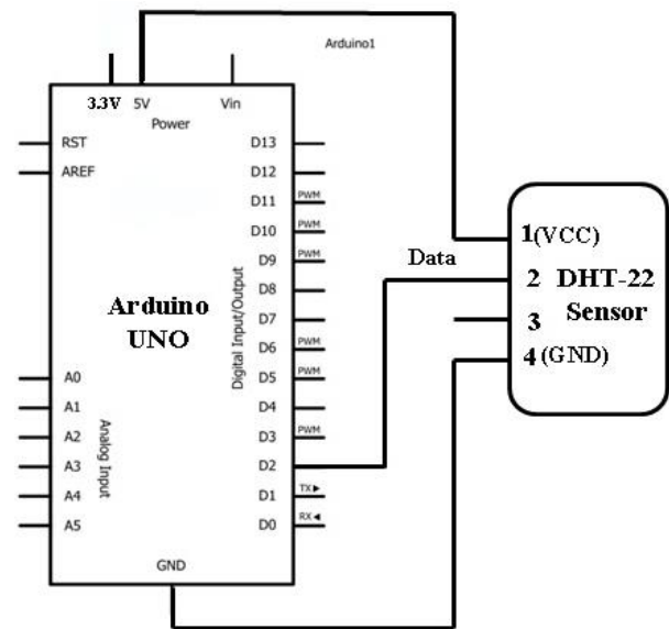
Fig. 8 Interfacing DHT-22 with Arduino Uno board.
