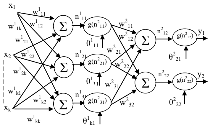
Fig.2 A multilayer perception network with one hidden layer
