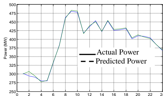
Fig.14 Actual and predicted Load profile for Wednesday 12/6/2013
