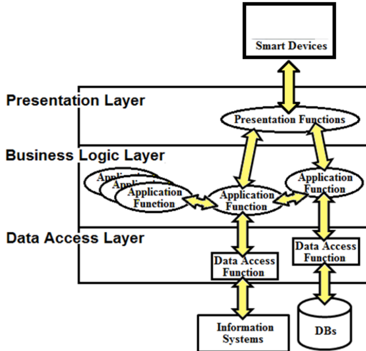
Figure (1) Mobile Application Server's Logical Layers.
