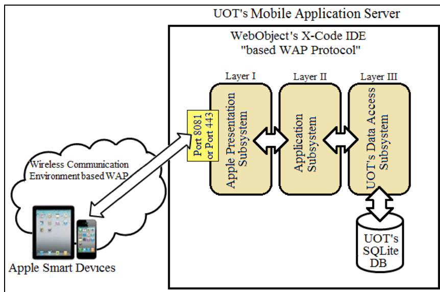
Figure (2) The Implemented Mobile UOT's Website Diagram.
