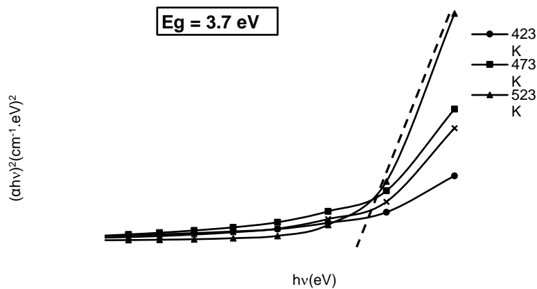
Figure (3): Plot of (\alpha h\nu)^2 against h\nu for indium oxide thin films at different substrate temperature.
