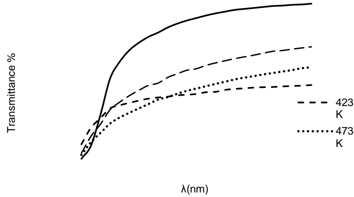
Figure (2): Transmittance spectra of the In 2 O 3 thin films in Different substrate temperature.
