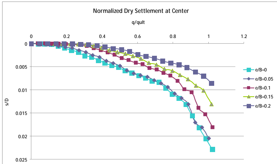
Figure (10) Normalized Pressure –Settlement Curves for Gypseous Soil at Dry State (Center).
