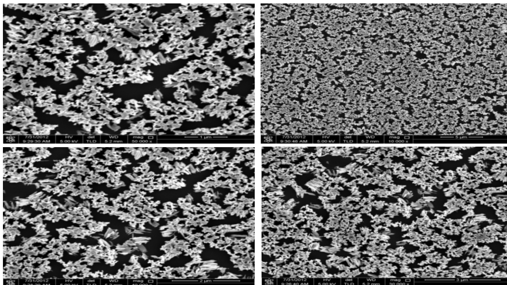
Figure 2: SEM surface morphology of ZnO layer grown on c-Si(111) substrate with many magnification power (1µm, 2µm, 3µm and 5µm)
