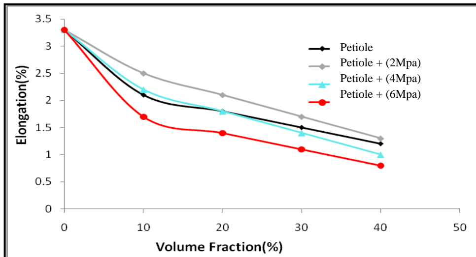
Figure (4): Elongation of polyester- composite as a function of Petiole date palm fiber content which subjected to various compression loads.
