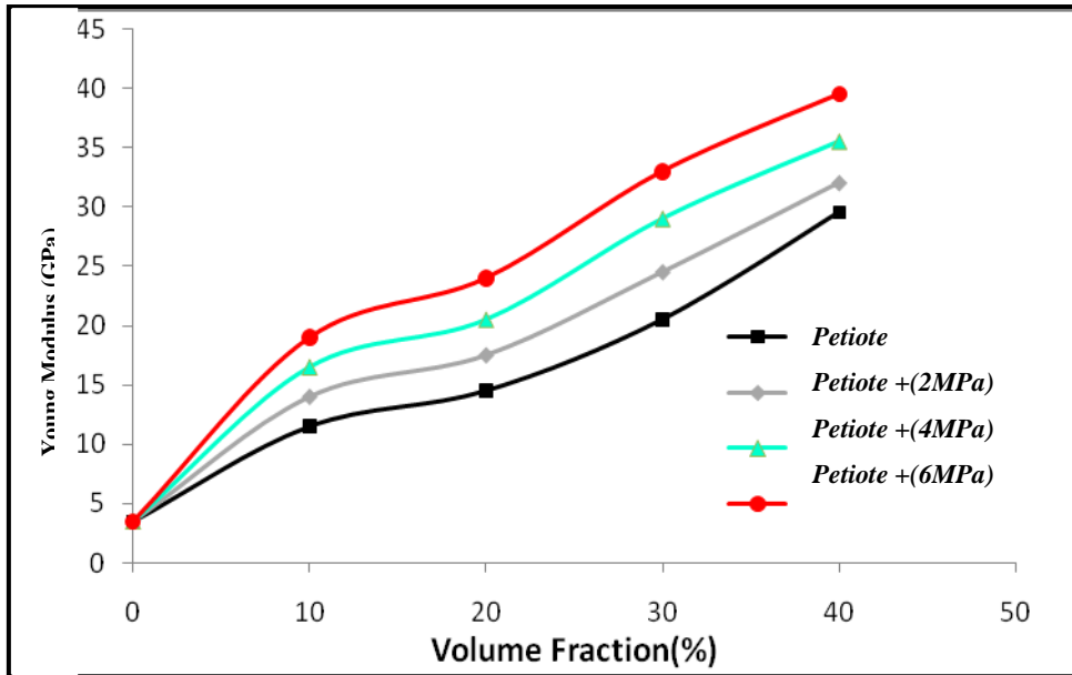
Figure (3): Young Modulus of polyester- composite as a function of Petiole date palm fiber content which subjected to various compression loads
