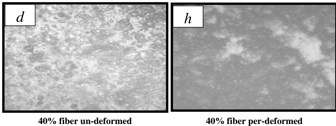
Figure. (12): Fractured Surface morphology of polyester-composite as a function of Petiole date palm fiber content (a,b,c,d un-deformed fibers)(e,f,g,h per-deformed fibers). 200x
