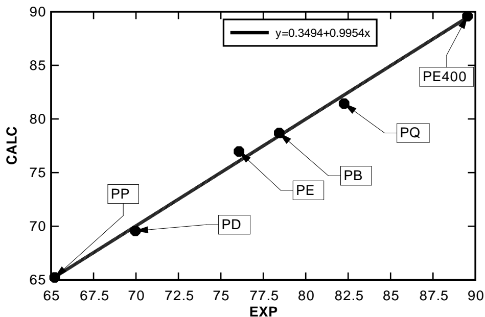
Fig. 4. Plot of the experimental ( T_g^{\circ}C ) vs. calculated ( T_g^{\circ}C ) of polymers using Eq 3.
