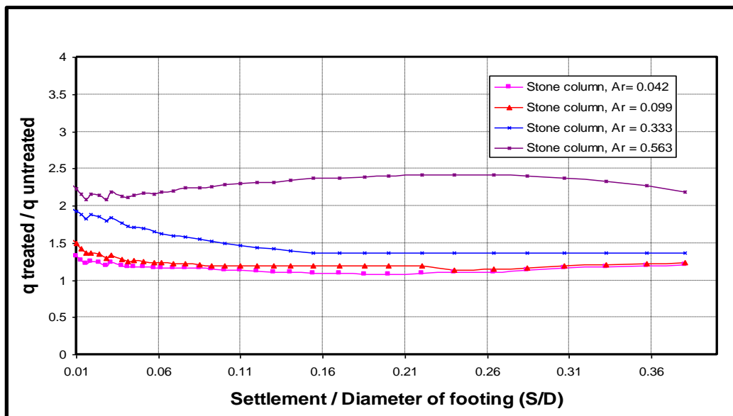
Figure (5): (q_{treated} / q_{untreated}) ratio versus (S/D) for the soil treated with stone columns, c_u= 11 kPa.
