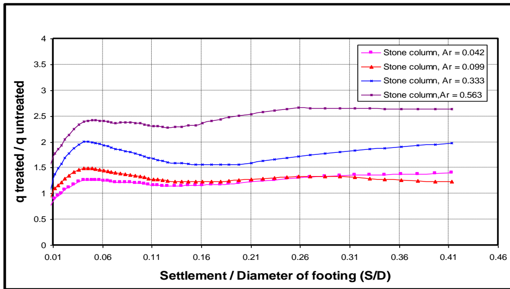
Figure (7): ( q_{treated} / q_{untreated} ) ratio versus (S/D) for the soil treated with stone columns, c_u = 16 kPa.
