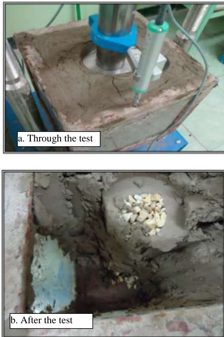
Figures (3) : Stone column model through and after the completion of the test
