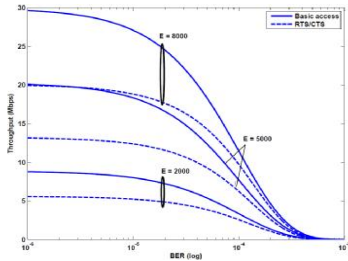
Figure (4): Throughput versus BER with different payload size and fiber delay = 22.24 \mu\text{s} .
