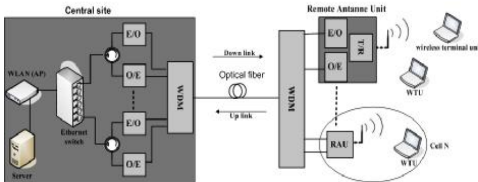
Figure (1) Block diagram for a WLAN over fiber network.
