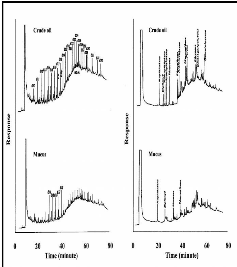
Figure 2. Capillary gas chromatograms of n-alkanes and aromatic hydrocarbons of Basrah regular crude oil and extract of petroleum hydrocarbons of the bivalve mucus.
