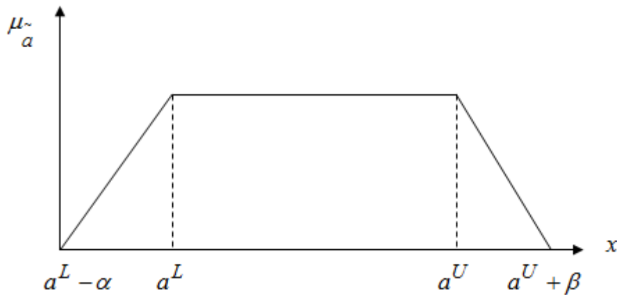
Figure 1 Trapezoidal fuzzy number
