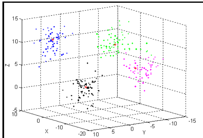
Figure (1) d-dimensional Euclidean space
