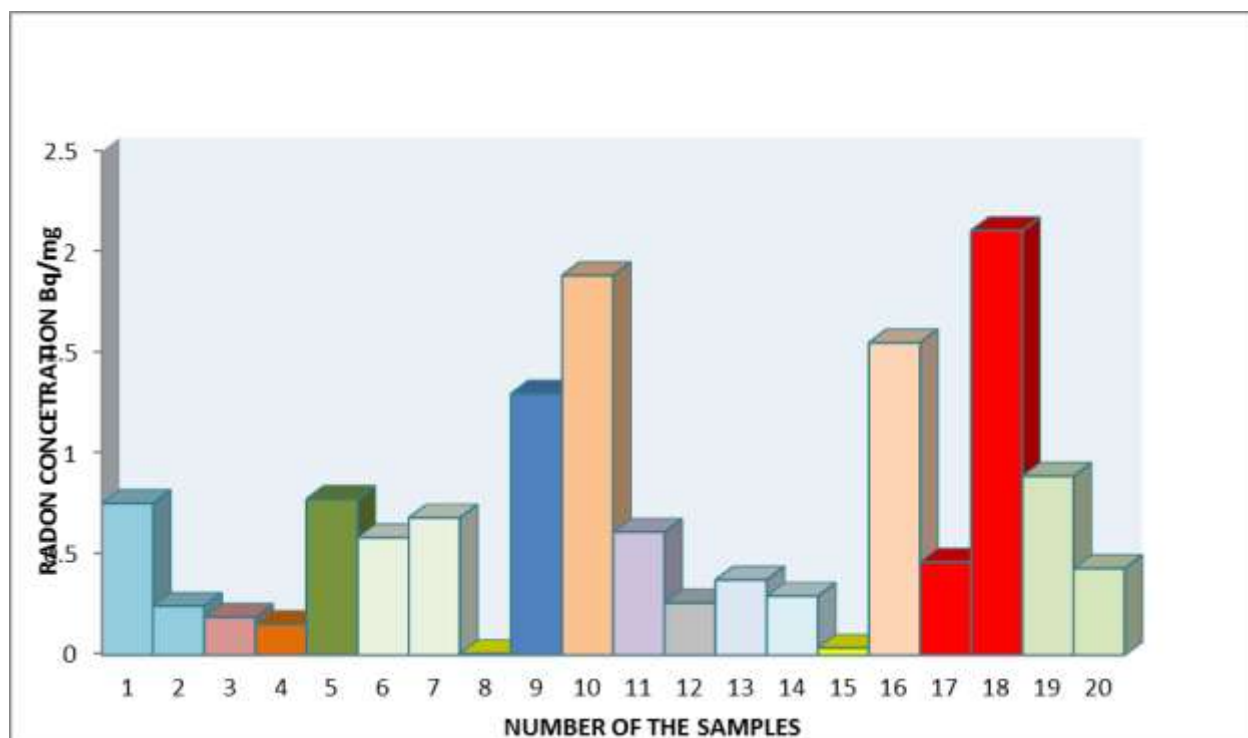
Fig. 2. Radon concentrations in twenty drugs samples from Iraq companies.
