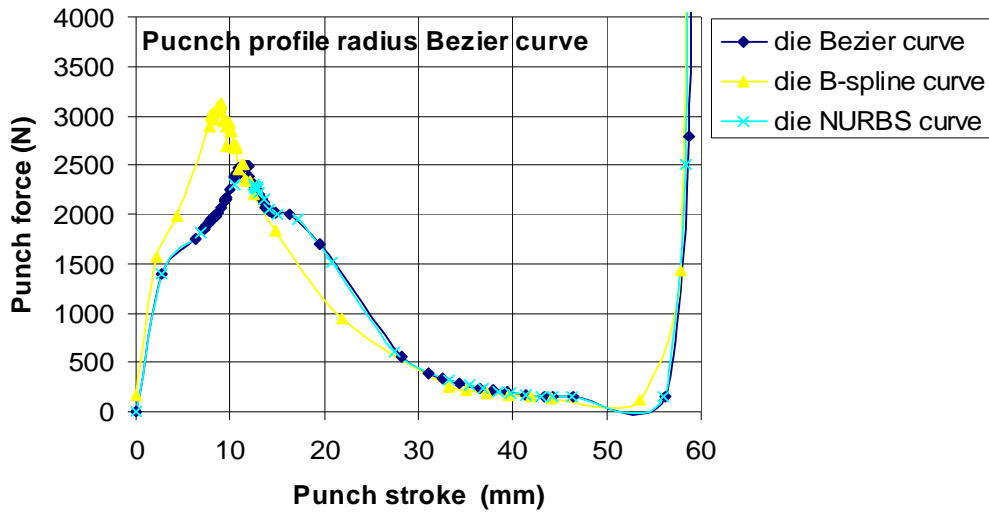
Figure (9) The effect of die profile on punch force
