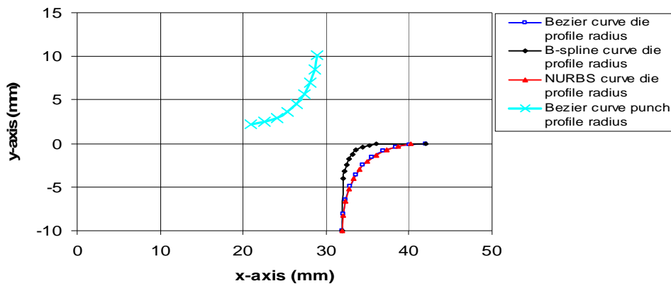
Figure (8) The die and punch profile by using free form surface.
