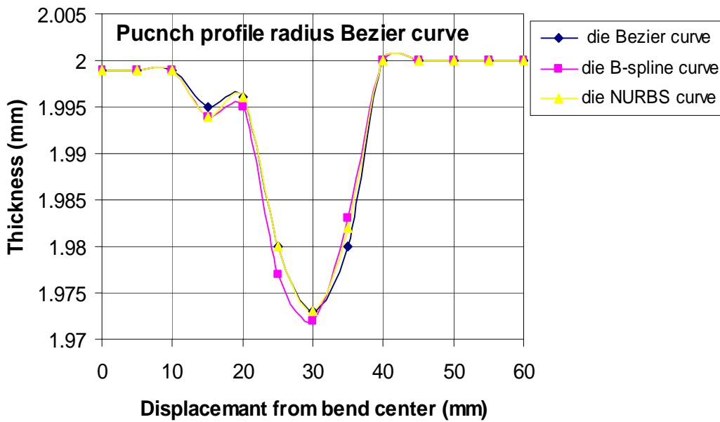
Figure (10) The effect of die profile on the wall thickness.
