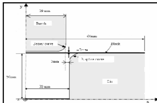
Figure (4).Schematic diagram of U-bending
