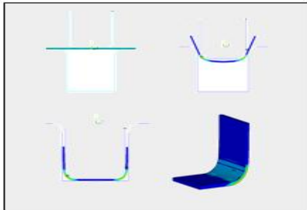
Figure (7) Sequences of U-bending
