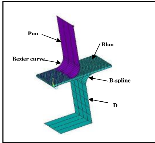
Figure (6) The finite element model of U-bending
