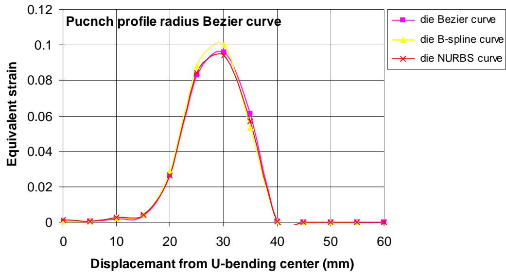
Figure (11) The effect of die profile on the equivalent strain.
