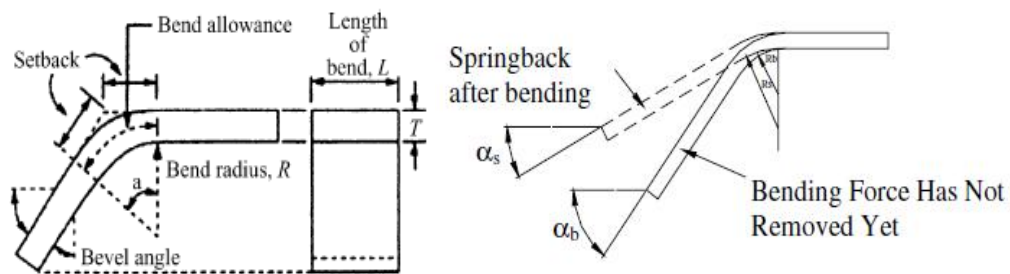
Figure (1) (a). Bending terminology, (b).Springback formed following bending [2, 3].
