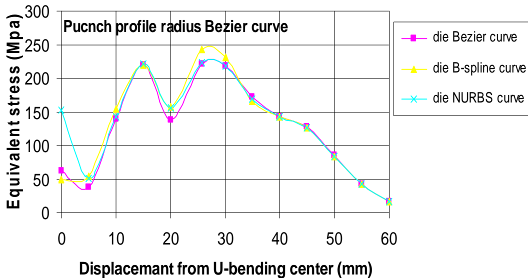
Figure (12) The effect of die profile on the equivalent stress.
