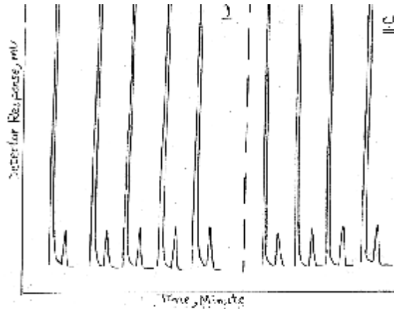
Figure (7) Chromatograms of methyl paraben extracted in two batches using Ethyl acetate from an insulin injection (Monotard) which was stored at freezing point for (6-7) days in (a) and for (9-10) days in (b) on 10%, OV-101 at 220C°.
