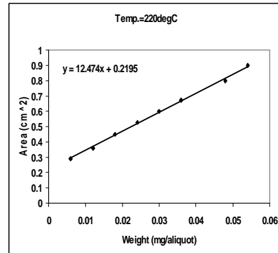
Figure (2) Standard calibration curve for methylparaben on 10% , 0V-101 at 220 C.
