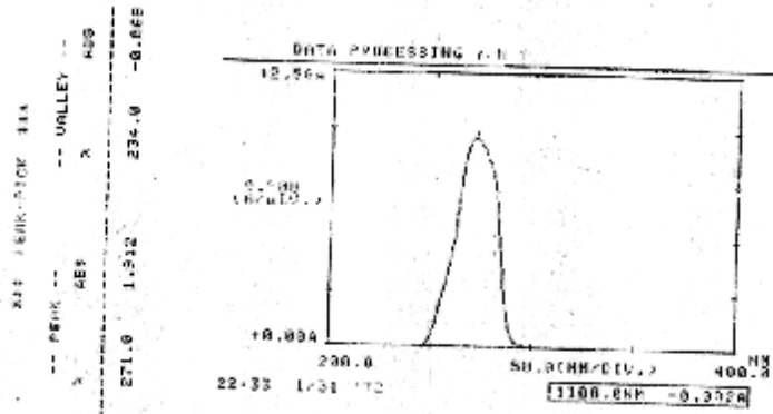
Figure (9)Ultraviolet absorption for meta-cresol from an insulin injection (Actrapid) extracted using ethyl acetate
