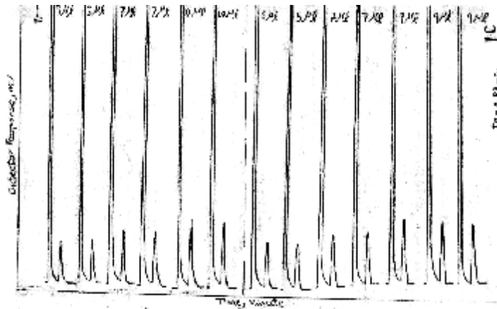
Figure (5) Chromatograms of methyl paraben extracted in two batches using Ethyl acetate from an insulin injection (Humulin), (a) from synthetic sample, (b) on 10%, OV-101 at 220C°.
