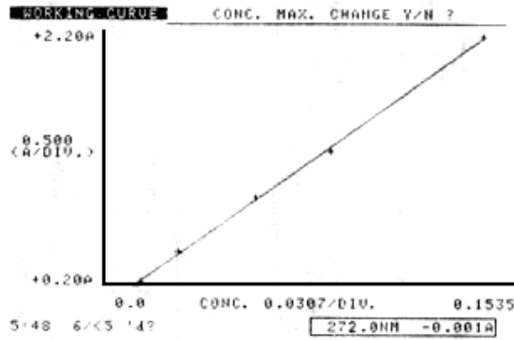
Figure (11) Standard calibration with curve for m-cresol by ultraviolet technique.
