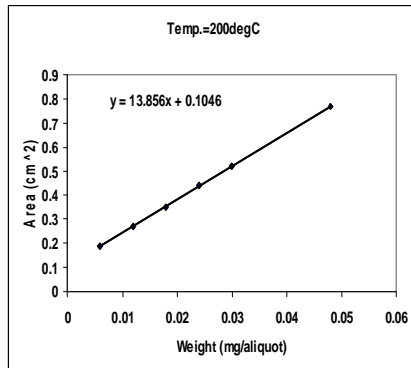
Figure (1) Standard calibration curve for methylparaben on 5% , 0V-101 at 200 C.
