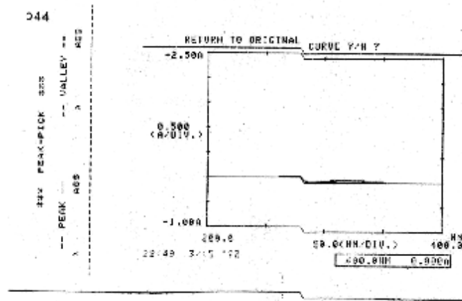
Figure (10) Ultraviolet absorption for meta-cresol from an insulin injection (Monotard) extracted using ethyl acetate after storing it at freezing point for 16 days.
