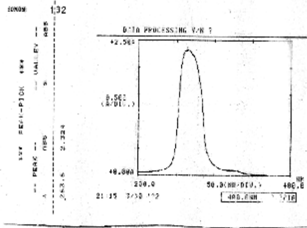
Figure (8)Ultraviolet absorption for methyl paraben from an insulin injection (Monotard) extracted using ethyl acetate .
