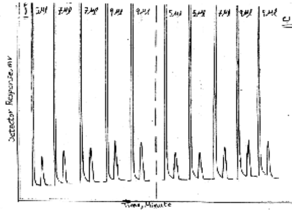
Figure (6) Chromatograms of methyl paraben extracted in two batches using Ethyl acetate from an insulin injection (Humulin) after its expiry date with (40-60) days in (a), (150-170) days in (b) on 10% OV-10 1 at 220C° which was stored at freezing point for (6-7) days in (a) and for (9-10) days in (b) on 10%, OV-101 at 220C°.
