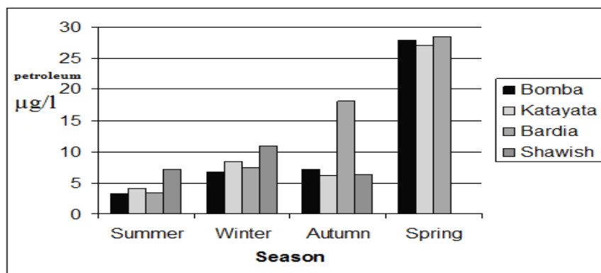
Figure 7. The seasonal variation of oil pollution for the studied coastal lagoons.
