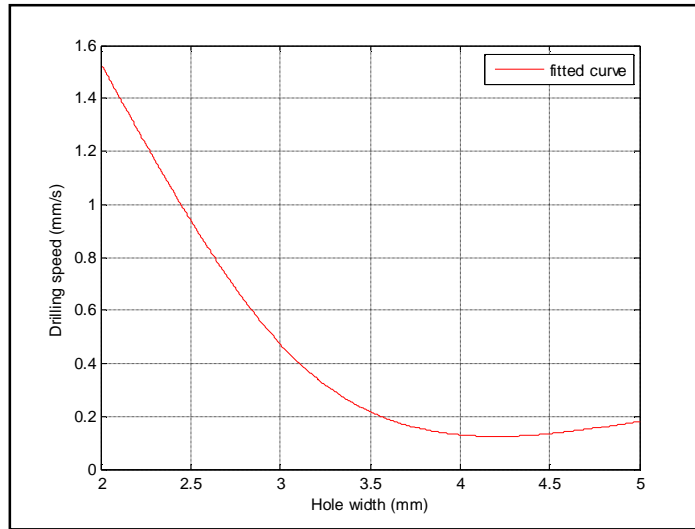
Figure (8) The relation between hole width and drilling speed for wood using CO 2 laser
