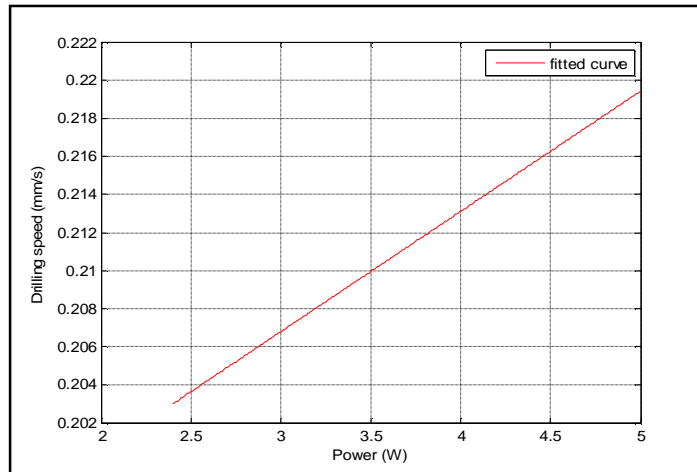
Figure (6) The relation between laser power and drilling speed for wood using CO 2 laser
