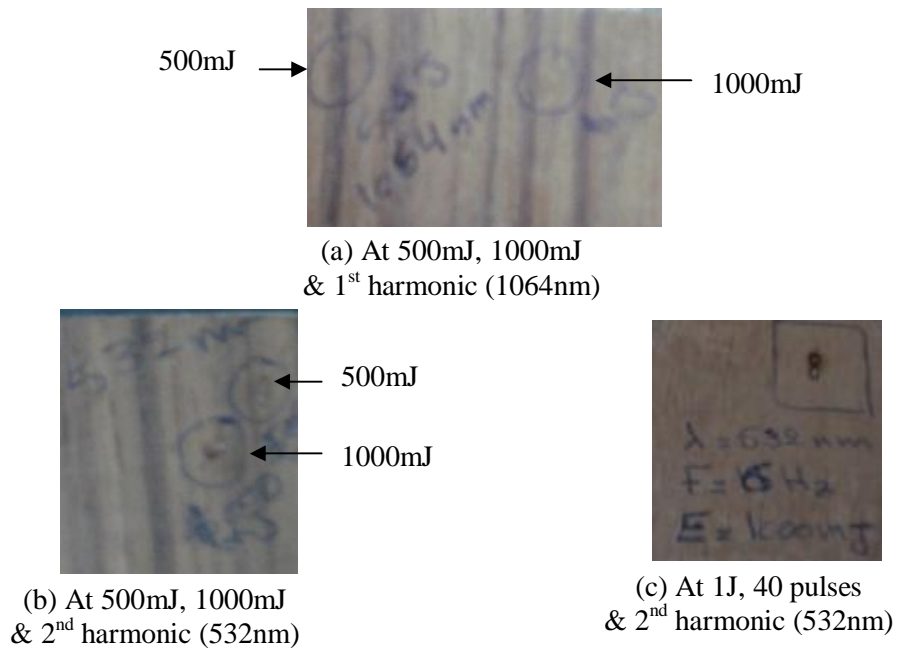
Figure (4) Wood drilled by Nd:YAG laser
