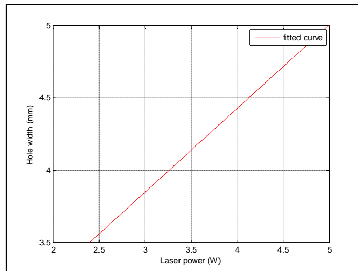
Figure (7) The relation between laser power and hole width for wood using CO 2 laser
