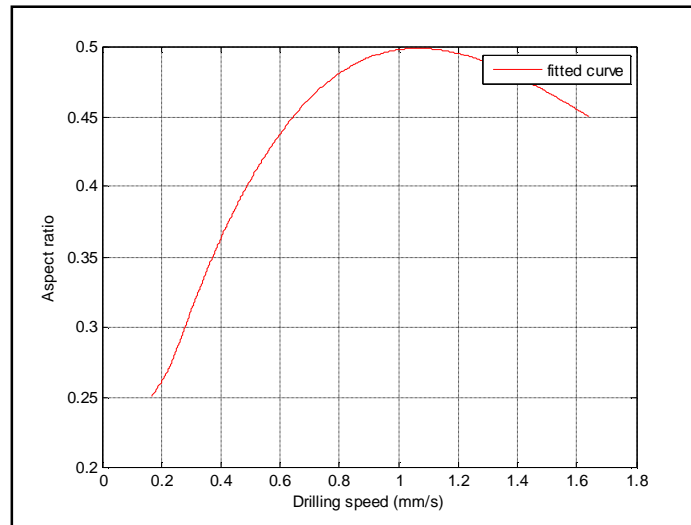
Figure (9) The relation between drilling speed and aspect ratio for wood using CO 2 laser
