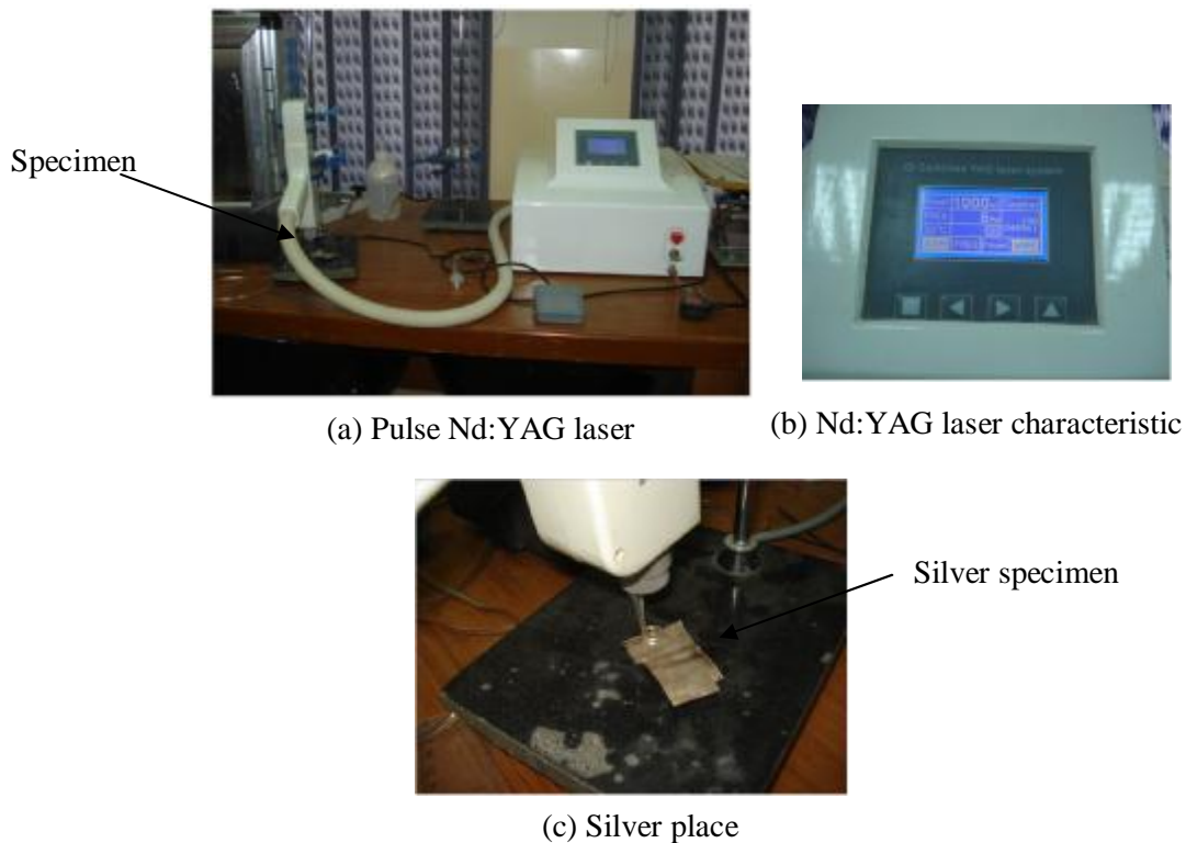
Figure (1) Setup used for silver drilling
