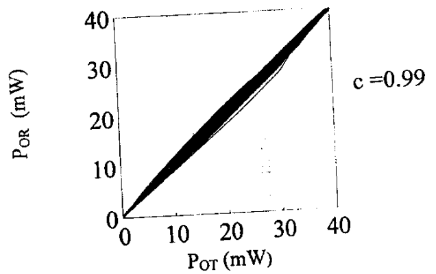
Figure (2): (a) Synchronization error \epsilon and (b) Correlation diagram of transmitter output vs. the receiver output from mismatch in feedback delay time \tau at different values of coupling strength c .
