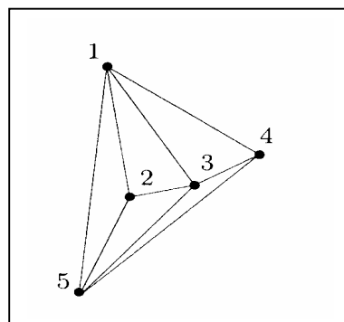
Figure (5.3) cyclic polytope C_3(5) .
