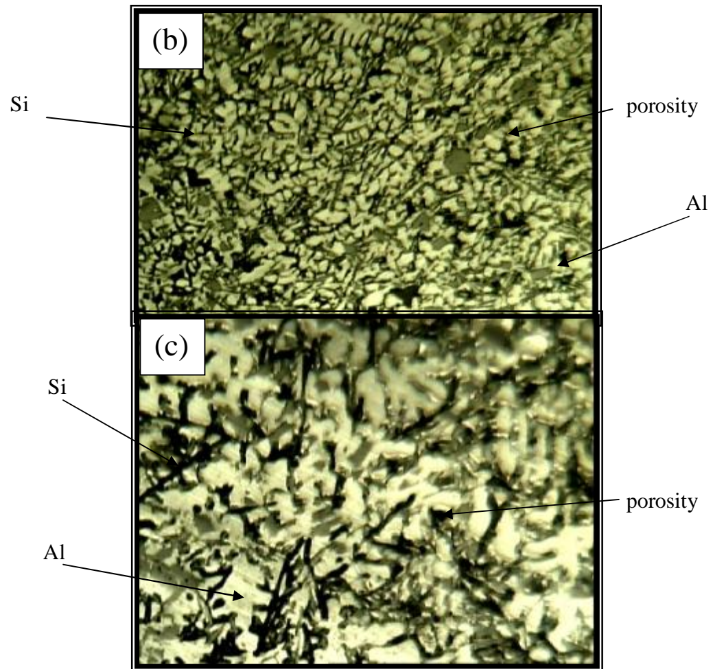
Figure (1) microstructure of as cast (a) Al-14% Si, (b) Al-14% Si-0.05% Na and (c) Al-14% Si-0.12% Na. X400.
