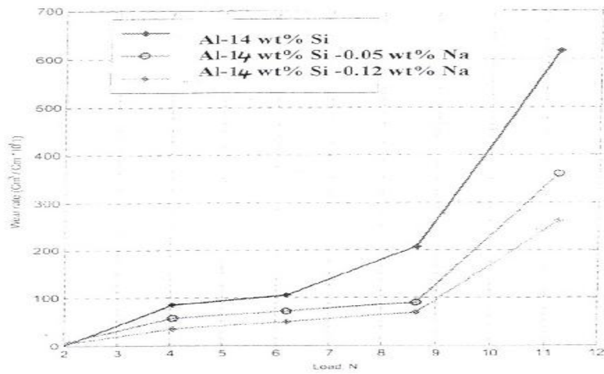
Fig 2. Wear rate- bearing load relationship for Al-Si alloys.
