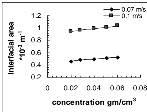
Fig(11) High electrolyte concentration vs. interfacial area at different superficial gas velocity.
