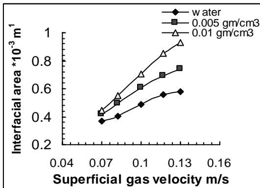
Fig.(2) Interfacial vs. area superficial gas velocity at different low electrolyte concentration and water.
