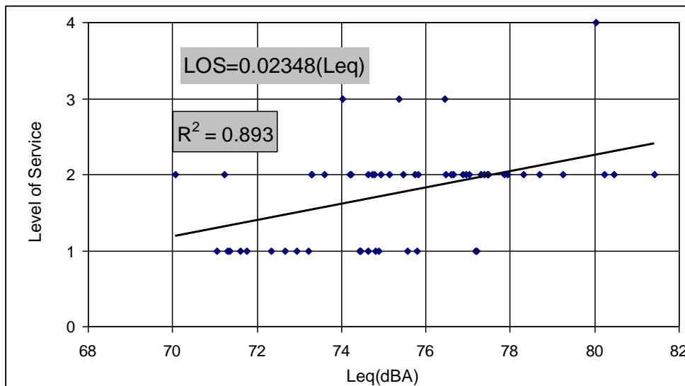
Figure (8) Traffic Equivalent Noise Level Against Level of Service For Selected Sections
