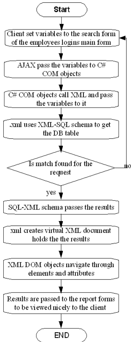
Figure (3): Employee Logins Procedure flow chart
