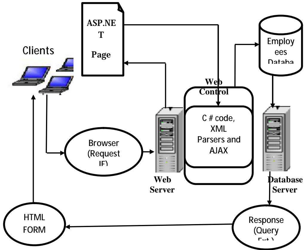
Figure (2): The proposed Three-Tier Web-Database Monitoring System.
