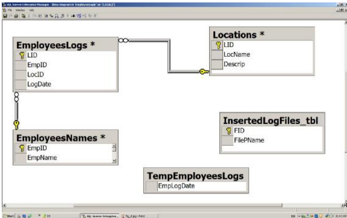
Figure (5): Employees Logins Database tables
