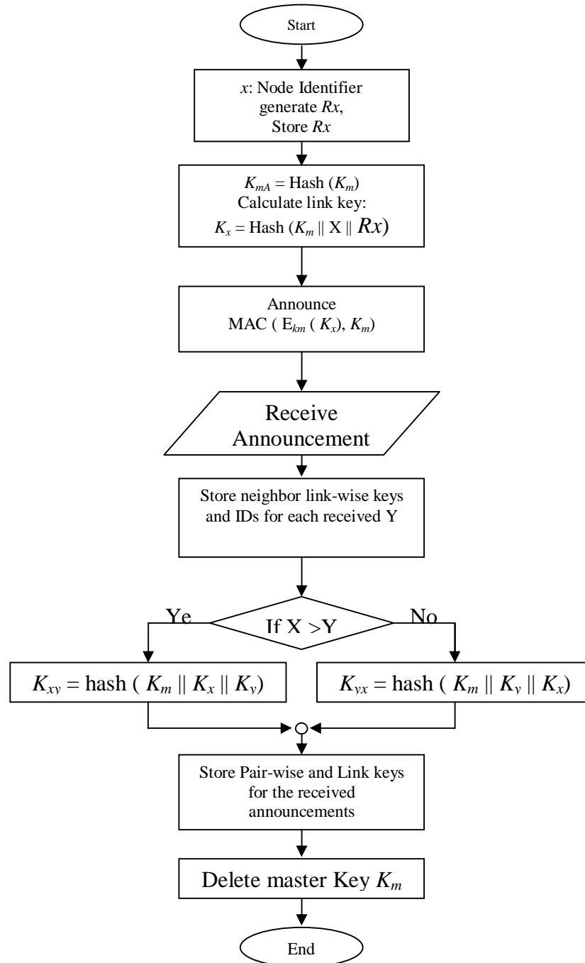
Figure (1) Key establishing flowchart.
