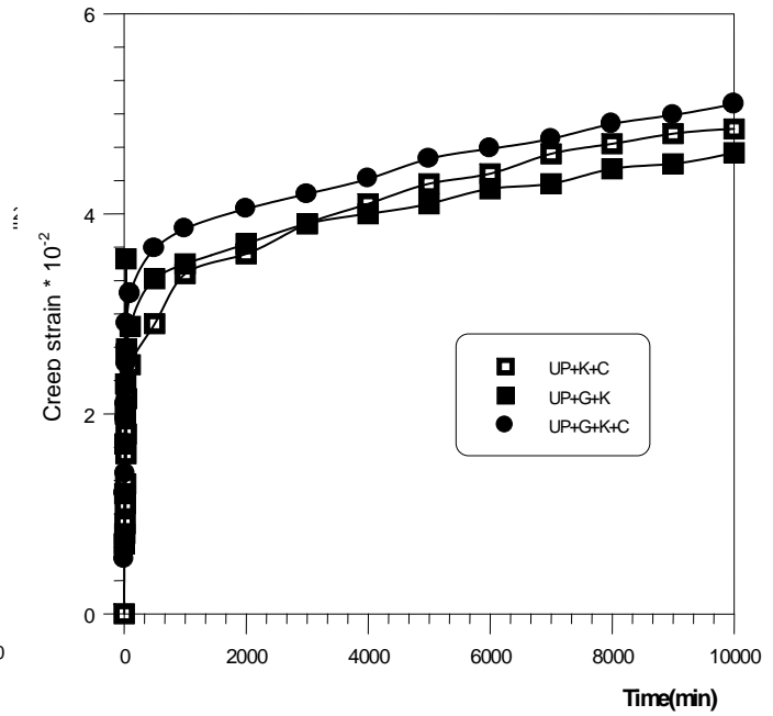
Fig (17) the variation of creep strain with time for UP composites (T = 25°C, hybrid)
