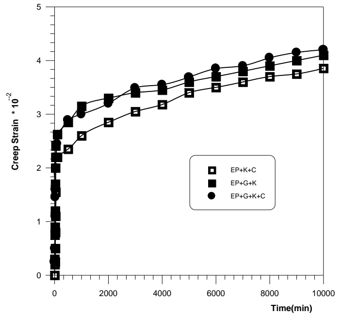
Fig (8) the variation of creep strain with time for EP composites (T = 25°C, hybrid)
