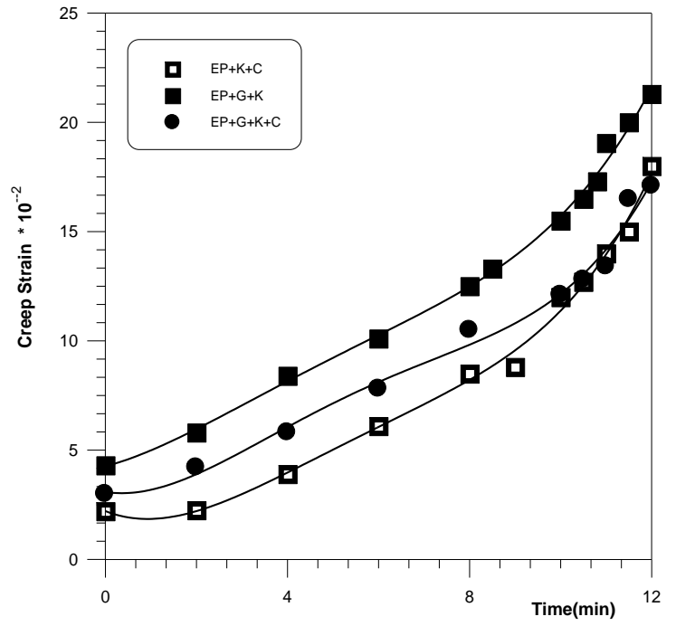
Fig (14) the variation of creep strain with time for EP composites (T = 70°C, hybrid)
