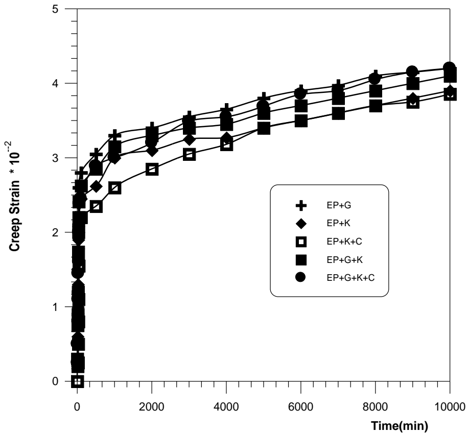
Fig (9) the variation of creep strain with time for EP composites (T = 25°C, single, hybrid)
