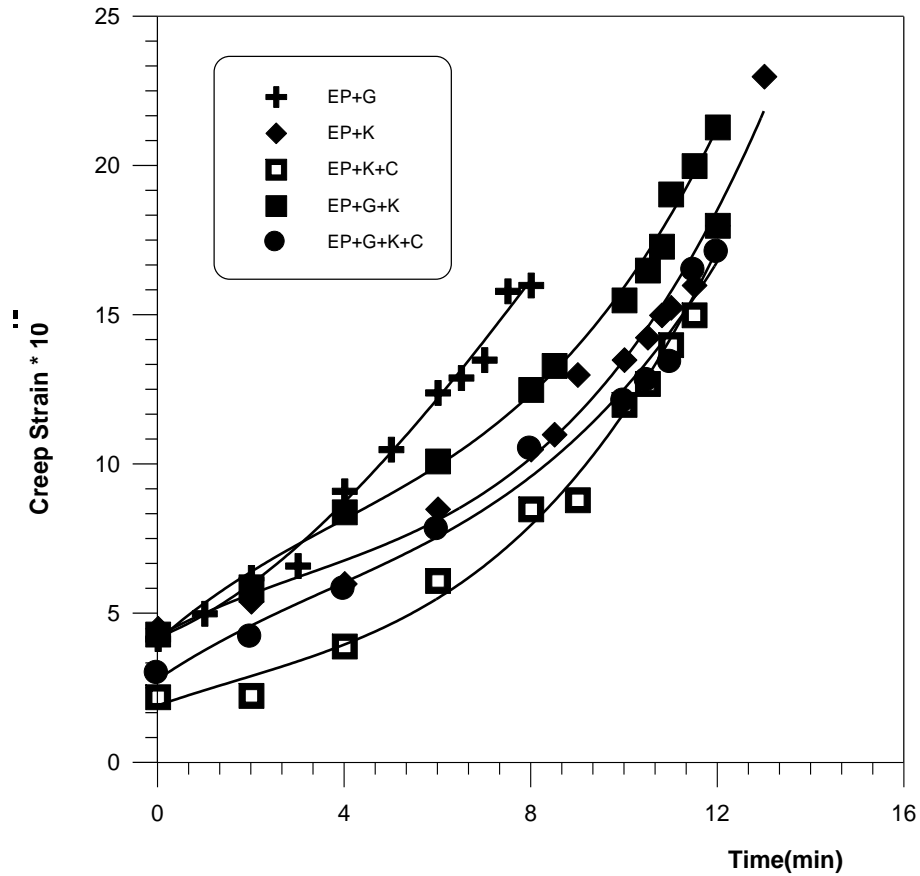
Fig (15) the variation of creep strain with time for EP composites (T = 70°C, single, hybrid)
