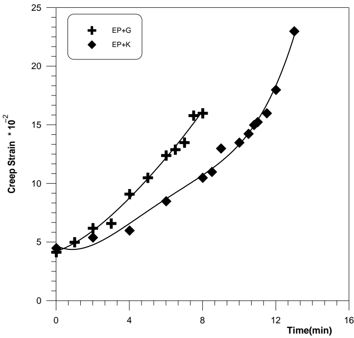
Fig (13) the variation of creep strain with time for EP composites (T = 70°C, single, hybrid)
