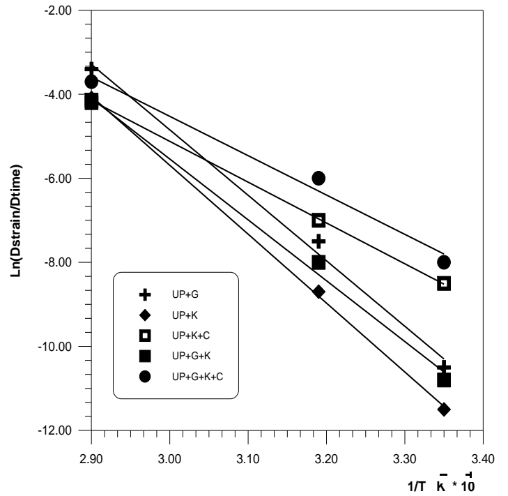
Fig (28) Ln (D strain / D time) versus 1/T plot for UP composites
