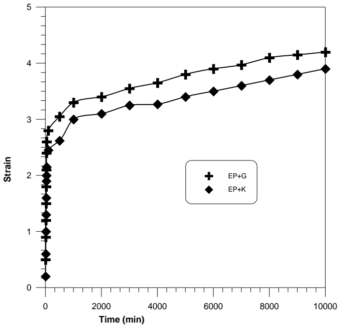
Fig (7) the variation of creep strain with time for EP composites (T = 25°C, single)
