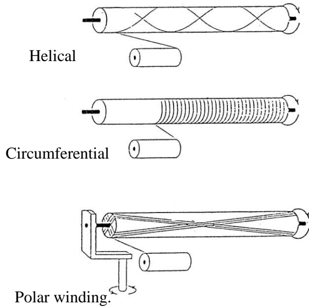
Fig. (1) Schematic representation of helical, circumferential and polar filament winding technique. [3]
