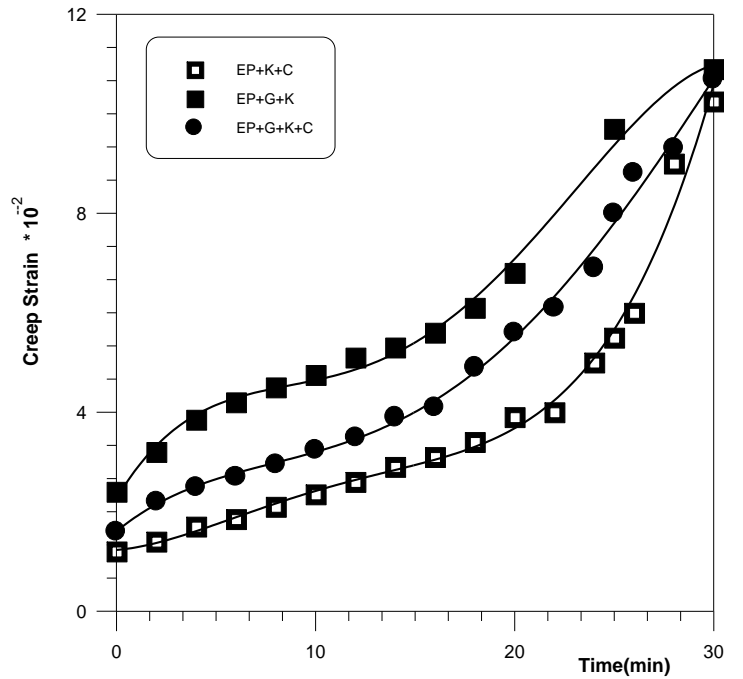
Fig (11) the variation of creep strain with time for EP composites (T = 40°C, hybrid)
