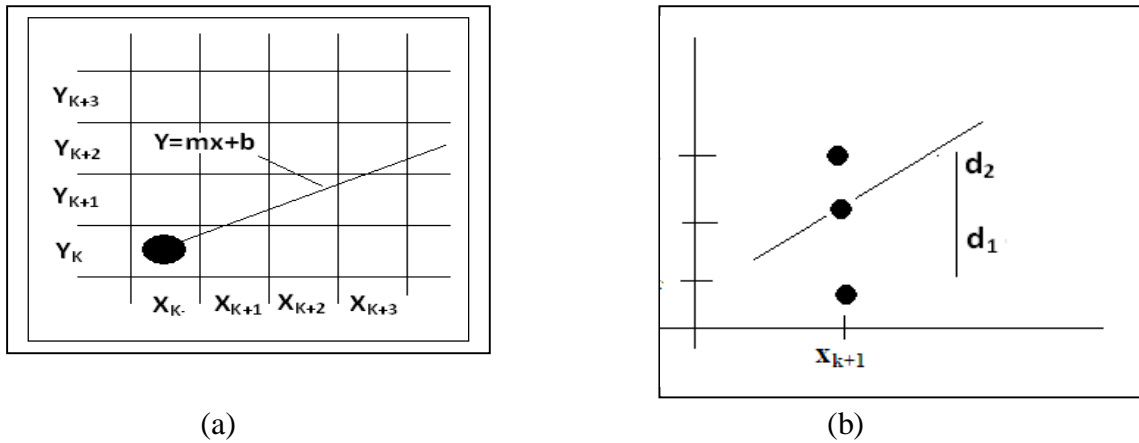
Figure (2) Section of the screen grid showing a pixel in on column x_k scan line y_k that is to be plotted along the path of a line segment with slope 0 < m < 1 .
