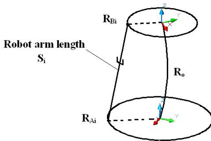
Figure3 Configuration System of the Robot Arm
