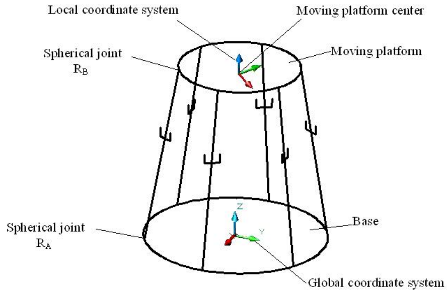
Figure 1 Gough – Stewart Parallel Robotic Mechanism
