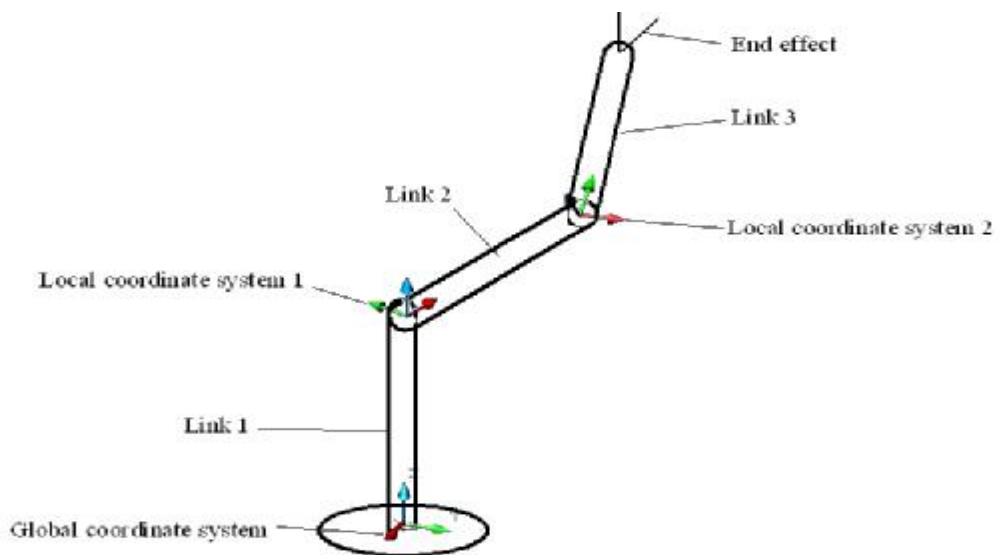
Figure 2 Open Kinematics Chain Mechanism
