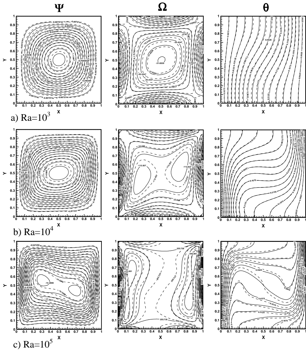
Figure (2): streamlines, vorticity lines and isotherms contours for pure fluid (solid lines) and nanofluids (dash lines) ( \phi=0.025 ) at different Rayleigh numbers.
