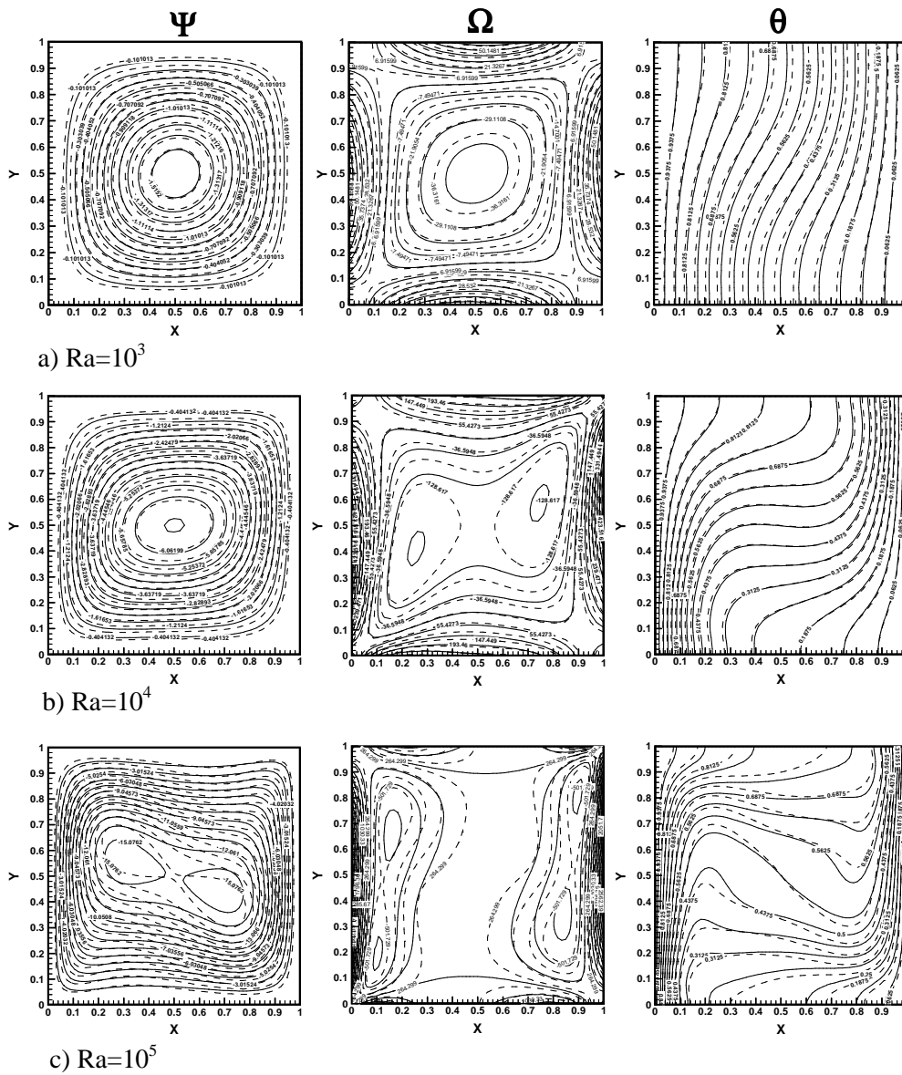
Figure (3): streamlines, vorticity lines and isotherms contours for pure fluid (solid lines) and nanofluids (dash lines) ( \phi=0.05 ) at different Rayleigh numbers.
