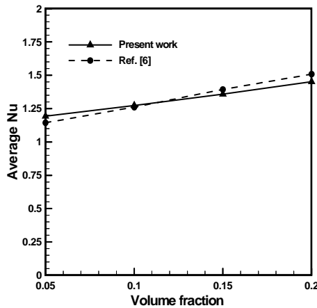
Figure (10): comparison between present work and Ref. [6] for relation between \overline{Nu} and \phi for Ra=10^3 . 2233
