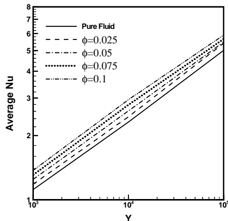
Figure (9): distribution of Nu at Ra=10^3 for pure fluid and nanofluids.
