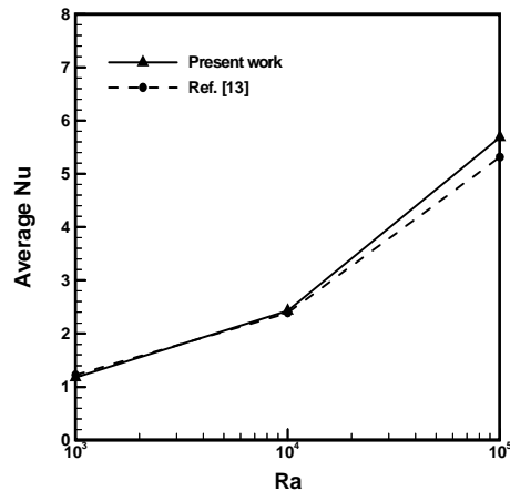
Figure (11): comparison between present work and Ref. [13] for relation between \overline{Nu} and Ra for \phi=0.04 .
