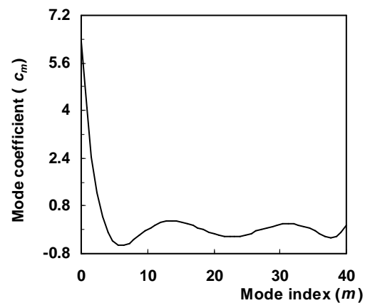
Figure (2) The analytical relation of the mode coefficient ( c_m ) to the mode index ( m ) within the examined values of beam propagation factor M^2=1-3
