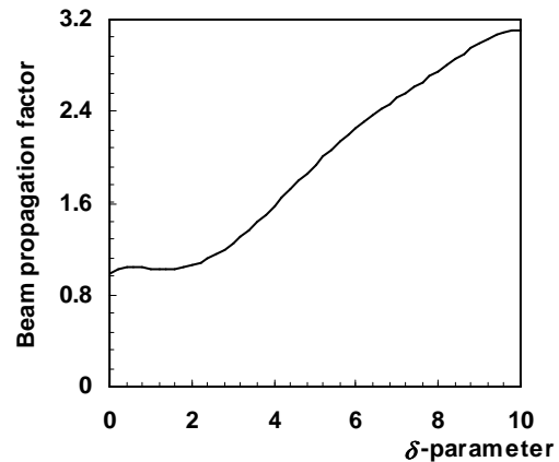
Figure. (1) Beam propagation factor ( M^2 ) of a hyperbolic Gaussian beam (e.g., laser beam) as a function of \delta
