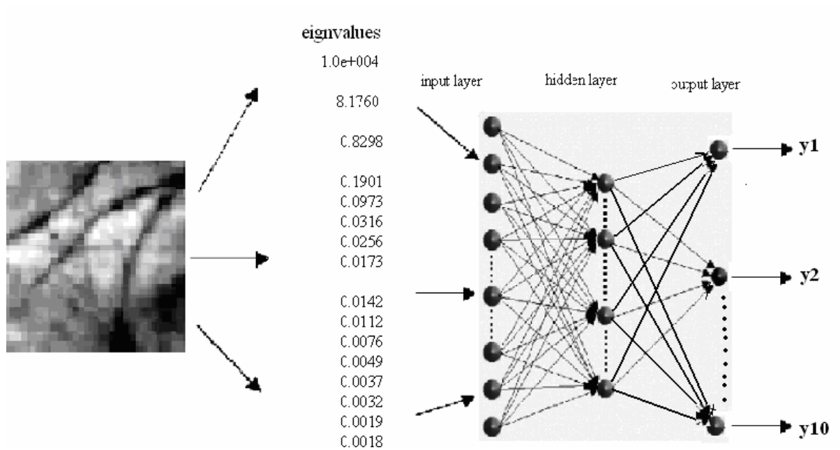
Figure 5 Backpropagation neural network (sigmoid activation function)
