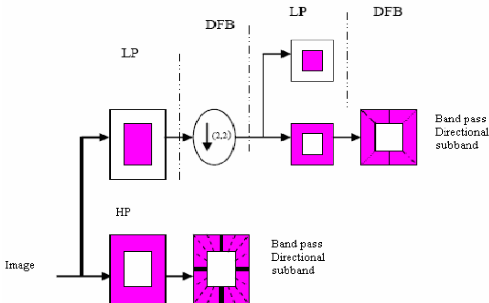
Figure 3 Double filter bank decomposition contourlet transform bands by the Laplacian pyramid is computed, and then a direction filter bank [10]
