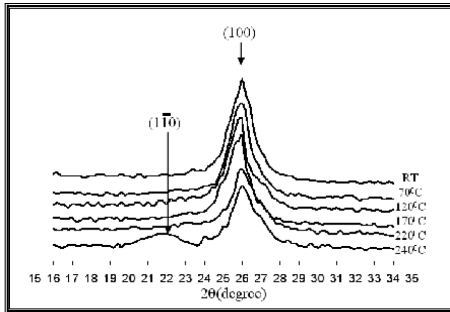
Figure (2) XRD profiles of Mylar films at different treatment temperatures.
