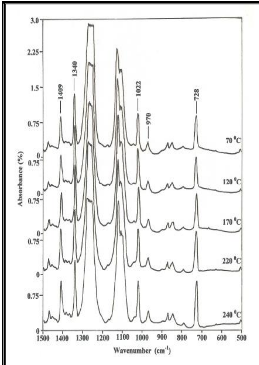
Figure (1) Absorbance FTIR spectra for heat treated Mylar films.
