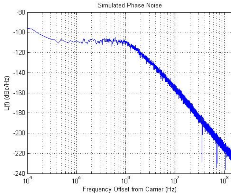
Figure (9): Simulation showing a phase noise.
