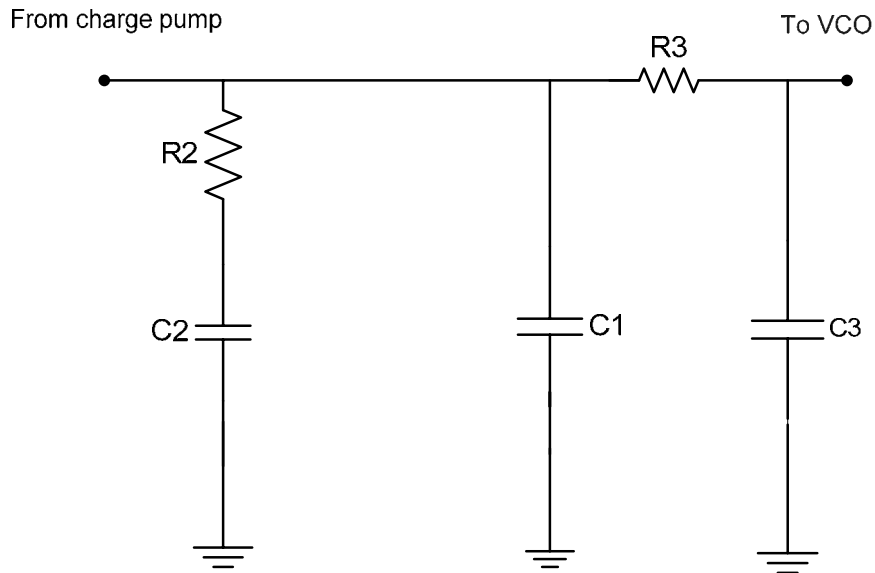
Figure (6): Second order lead-lag loop Filter with added pole.
