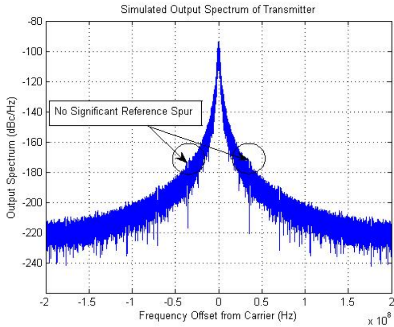
Figure (10): Output spectrum of PFD/DAC synthesizer for 2.566GHz.
