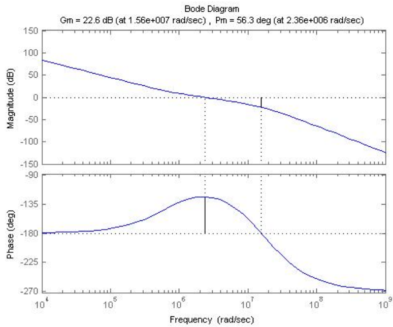
Figure (11): Simulation showing open-loop response.
