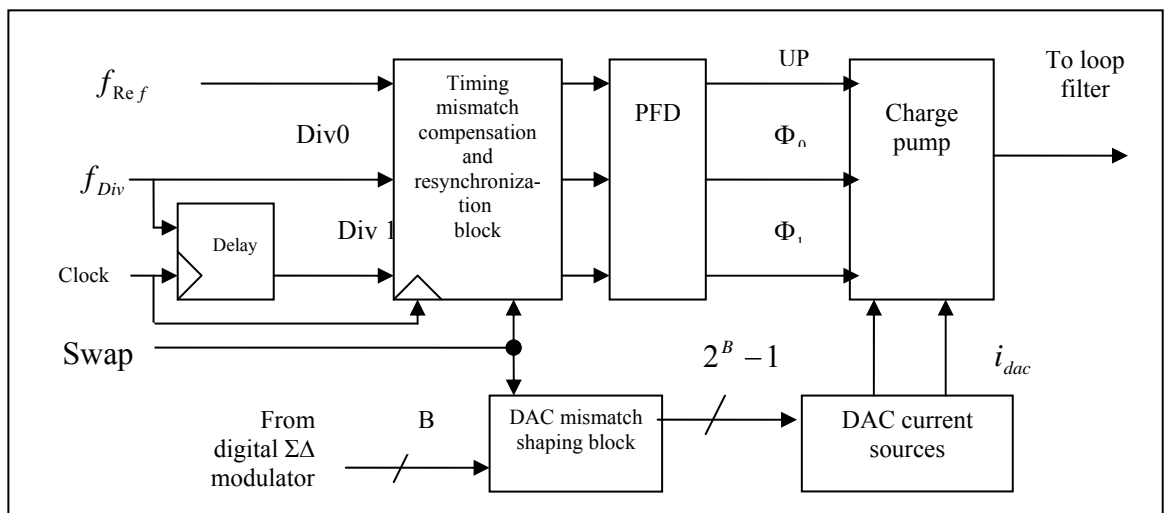
Figure (5): PFD/DAC block diagram.
