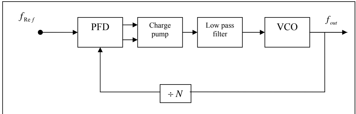
Figure (1): The block diagram of phase-locked loop.
