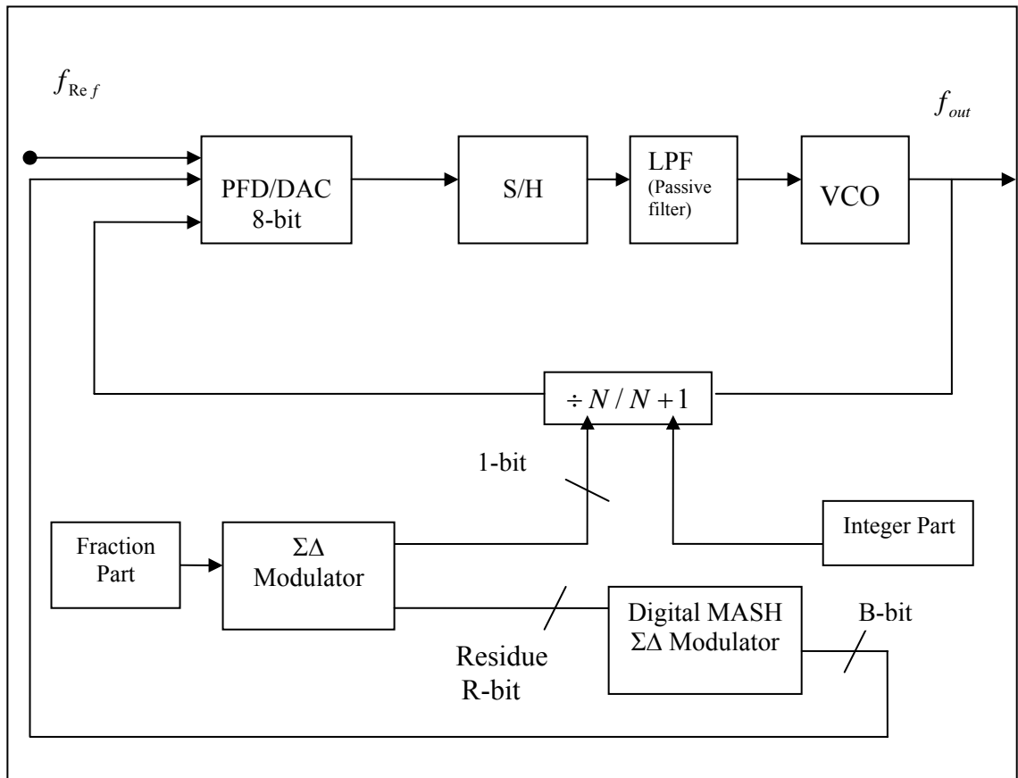
Figure (4): Sigma-delta technique with hybrid PFD/DAC structure.
