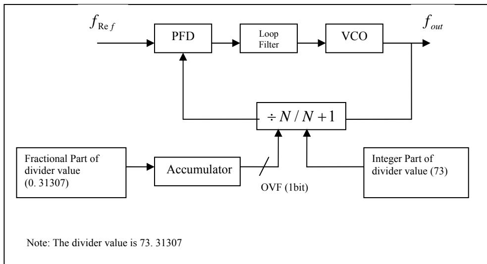
Figure (1): The block diagram of phase-locked loop.
