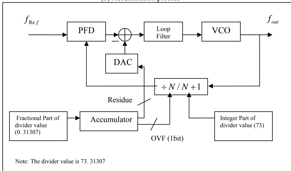
Figure (2): (a) Classical fractional-N synthesizer (b) Accumulation process
