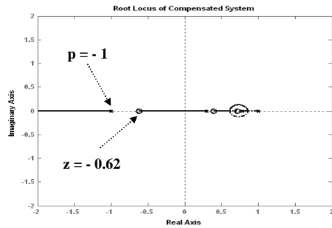
Fig. 24: Root locus of the compensated system with discrete PID controller
