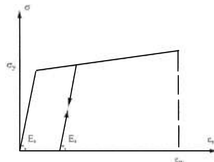
Fig. (5). Stress-strain relationship of steel bars used in the analysis.
