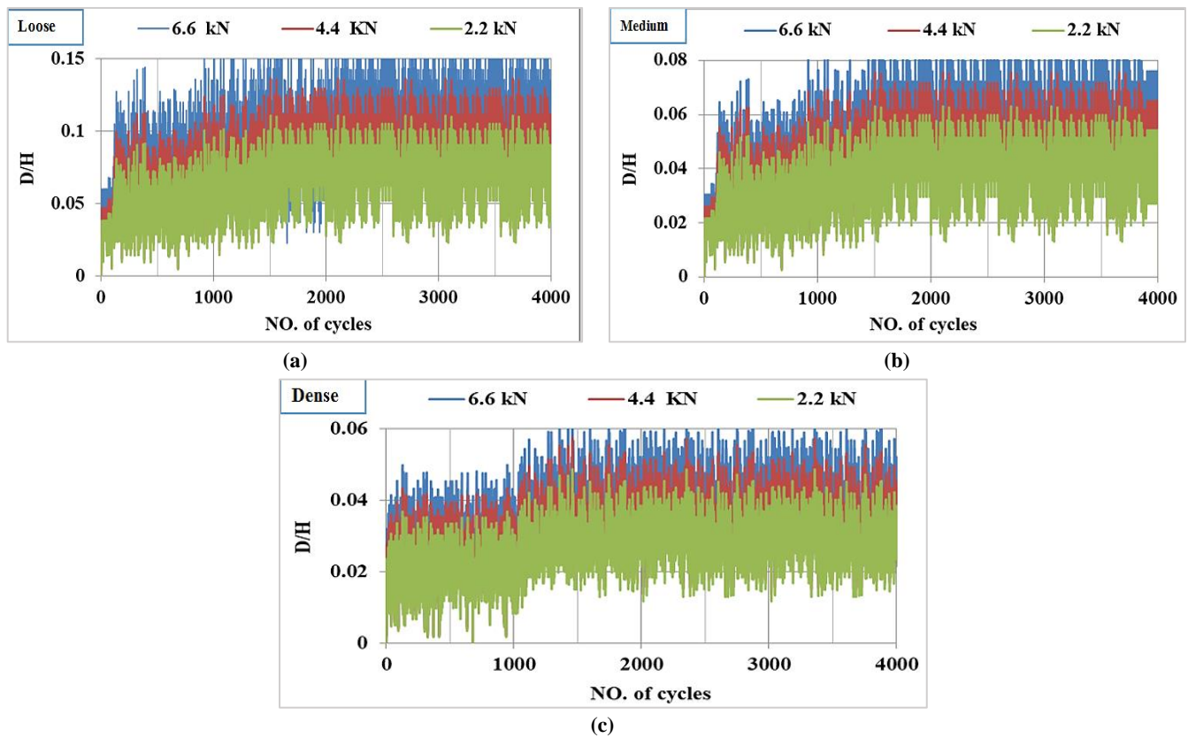
Figure 9: Cyclic number versus lateral wall displacement ratio D/H with different load amplitude for X = 0.5 H , under 2 Hz frequency; a., b, and c for loose, medium, and dense sand, respectively.
