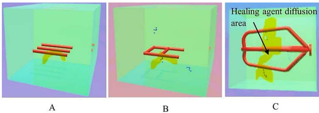
Figure 1: Shows a specimen with a vascular tube with different design in cube (a) a one, (b) two, and (c) three-dimensional
