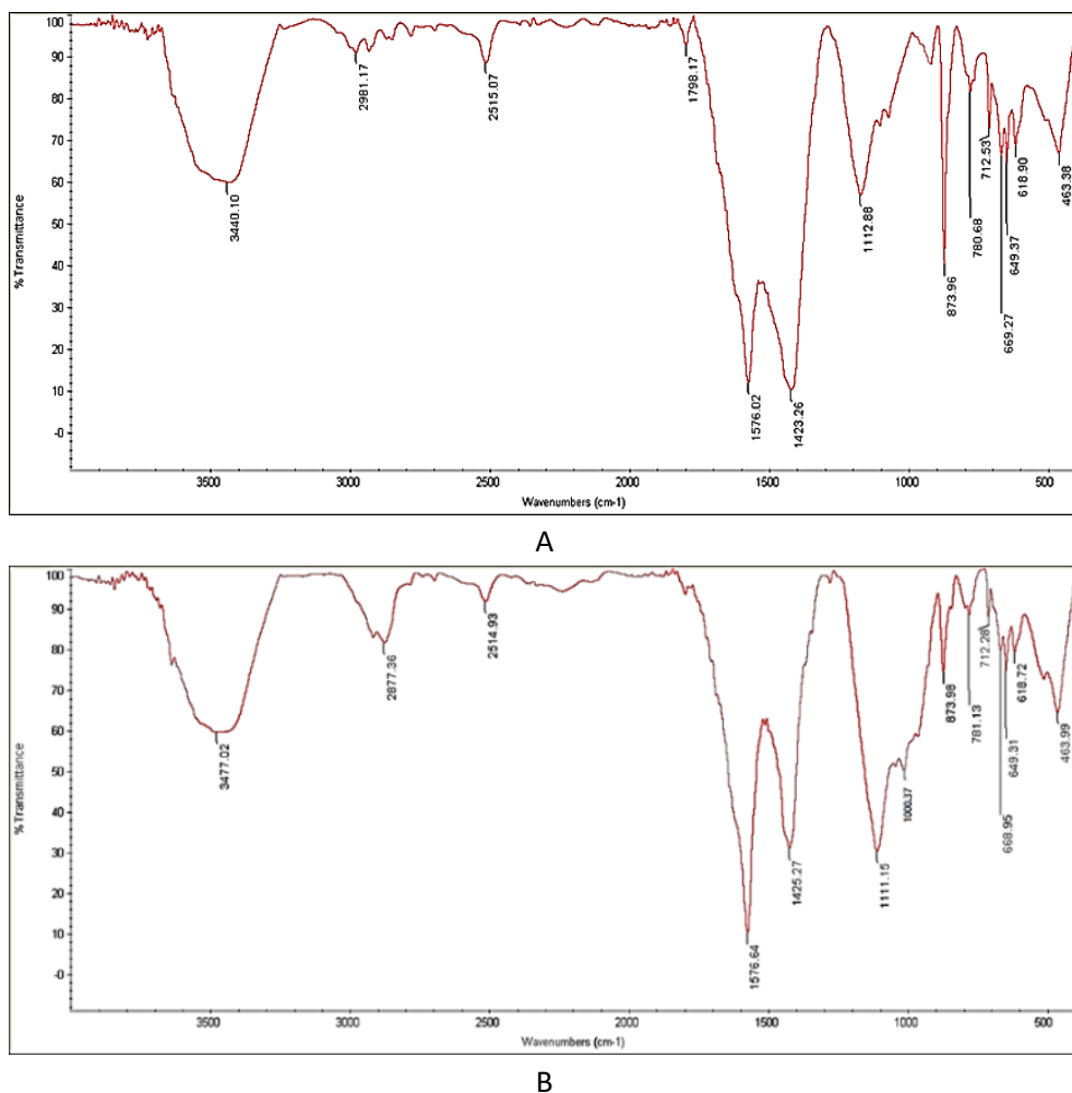
Figure 7: FTIR spectra of (a) the control sample and (b) the sample after the healing period
