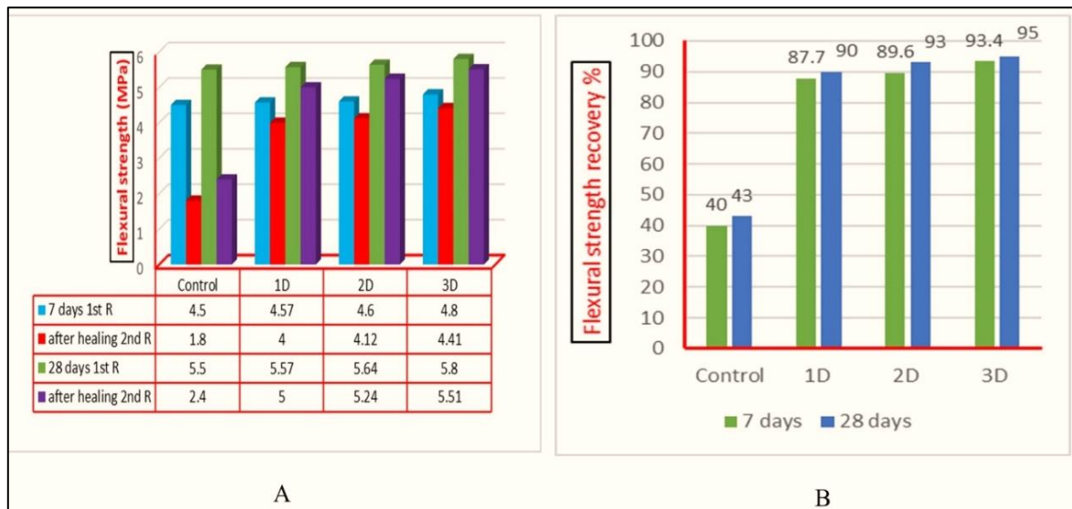
Figure 5: Concrete flexural strength with varied vascular tube designs (a) Each sample has a unique design at 1st R and 2nd R (b) Flexural strength percentage recovery of sample with differend design vascular tube.
