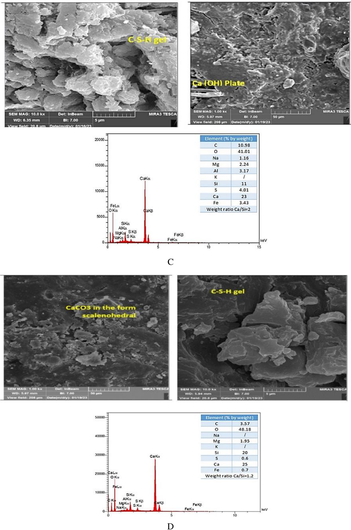
Figure 6: Visualizes the pre- and post-self-healing images of cementitious materials captured using (SEM-EDS), (a) the SEM-EDS image of cementitious materials at the 7 day, before they undergo self-healing, (b) the SEM-EDS image illustrates the cementitious materials following healing period, (c) cementitious materials before they self-heal, as seen in the SEM-EDS image taken at 28 days from curing, (d) after 28 days of healing period, the cementitious materials are seen in the SEM-EDS photo
