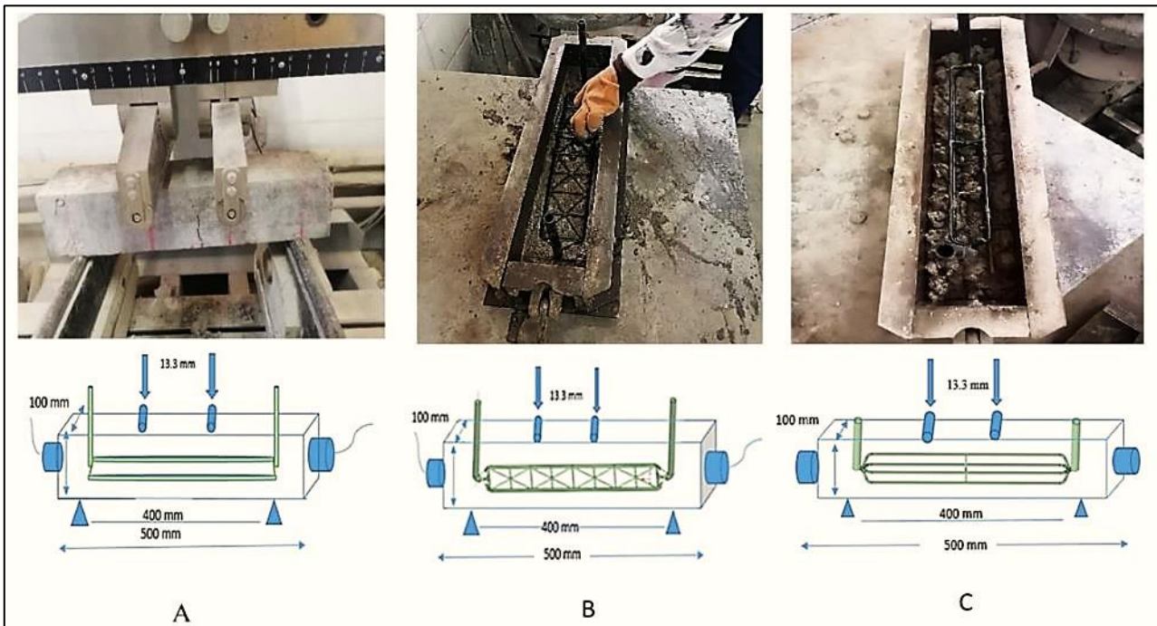
Figure 2: Displays a prism specimen with embedded a vascular tube that has been placed in three different dimensions (a) 1D, (b) 2D, and (c) 3D
