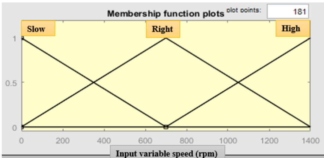
Figure 5: I/P membership (s peed)
