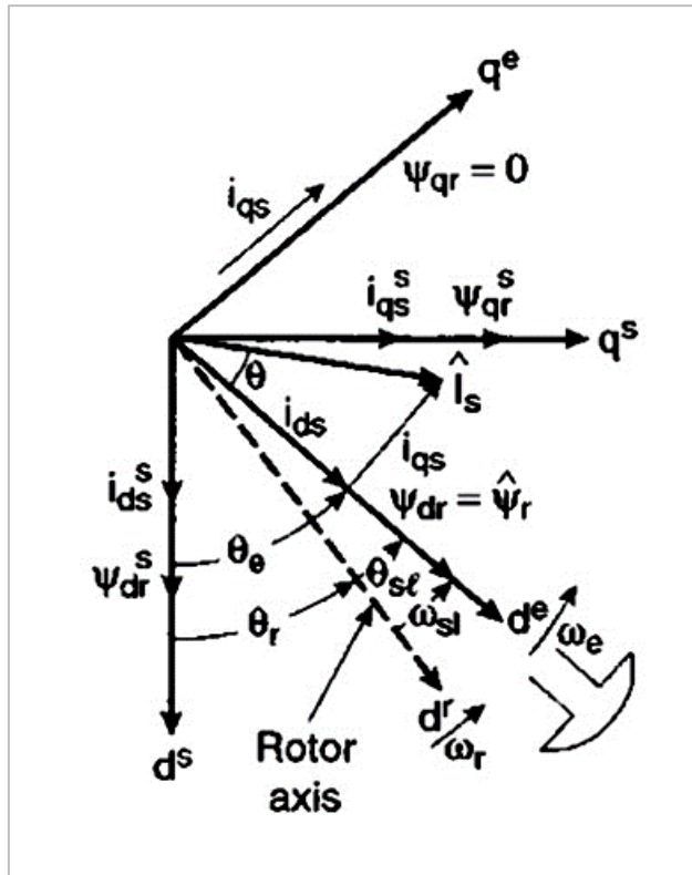
Figure 3: Phasor diagram indirect vector control method of Induction motor [48]
