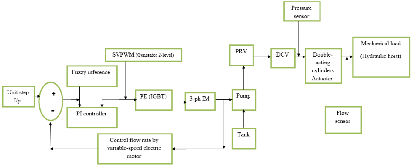
Figure 1: PI-fuzzy control of electro-hydraulic system
