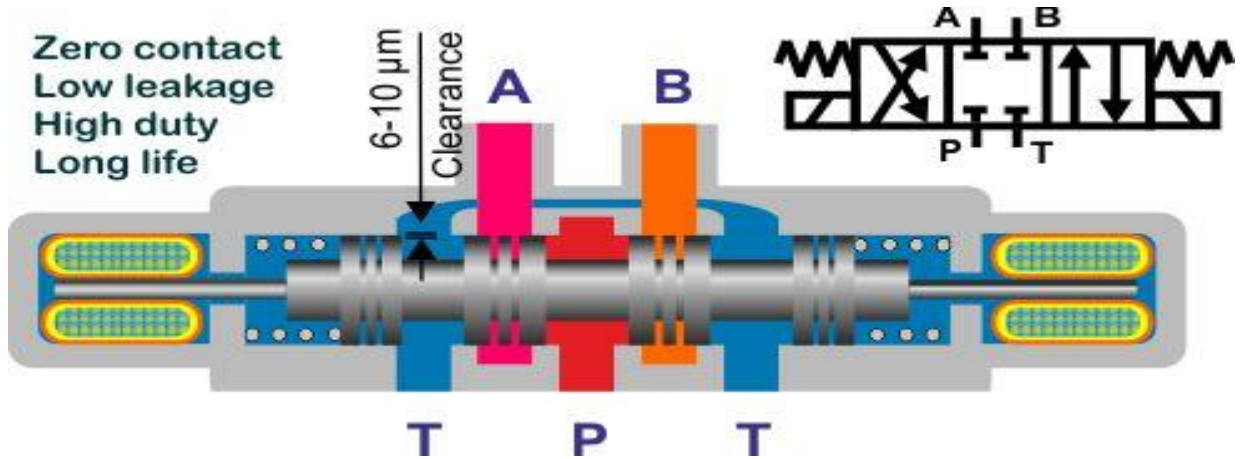
Figure 2: Directional control valve [42]
