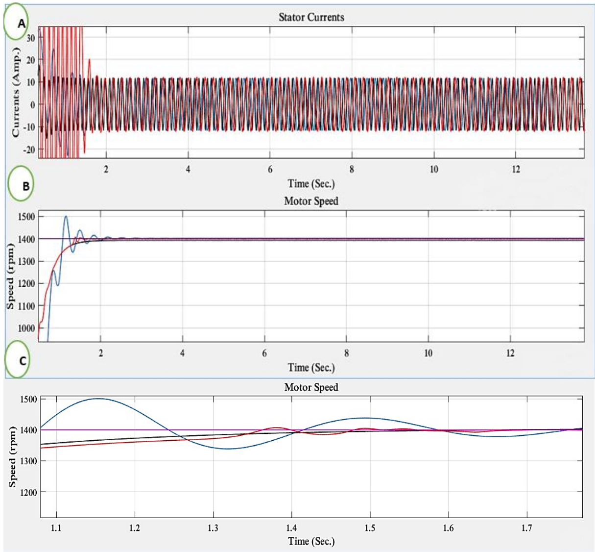
Figure 12: Dynamic response of motor currents and speeds for three control techniques
