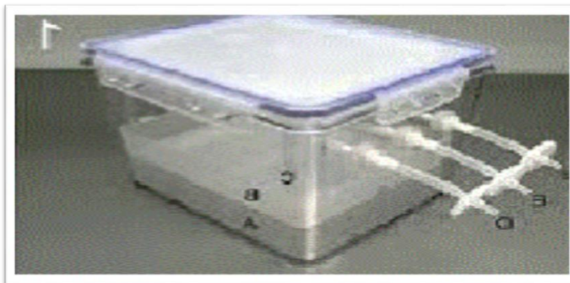
Main parts of Plate form bioreactor system
