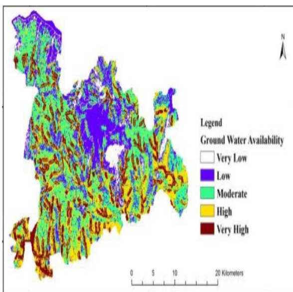
Figure.7 map shows areas of different groundwater potential
