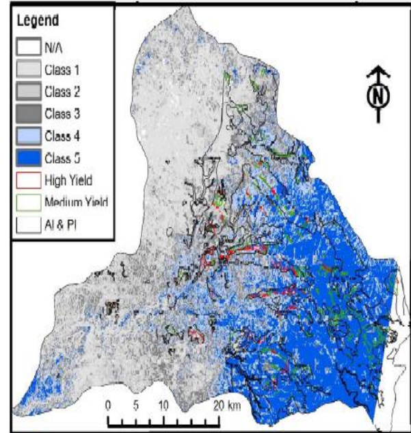
Figure 5. map shows distribution of alluvial fan
