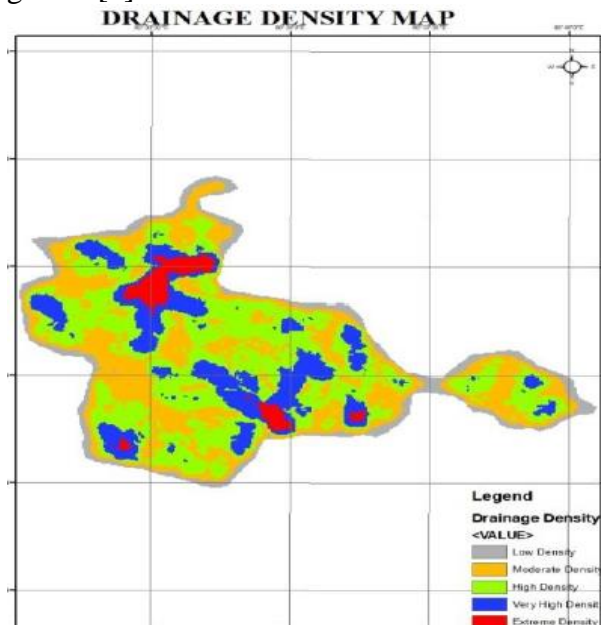
Figure .4 map reveals drainage density
