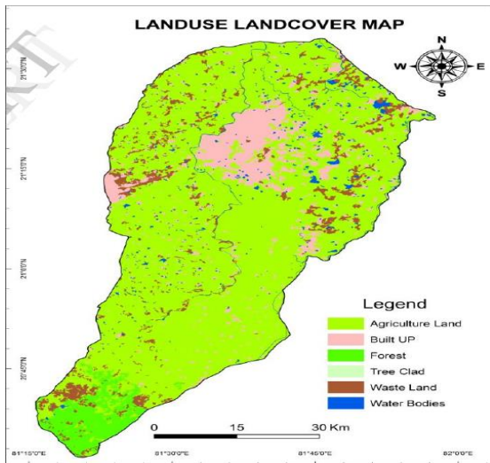
Figure .6 map reveals land cover classes
