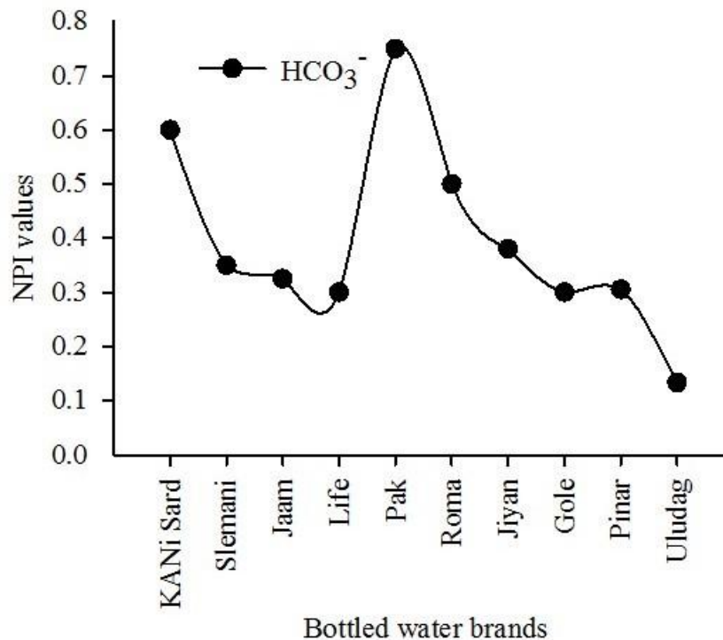
Figure 5: The variation of NPI values of HCO 3 - .
