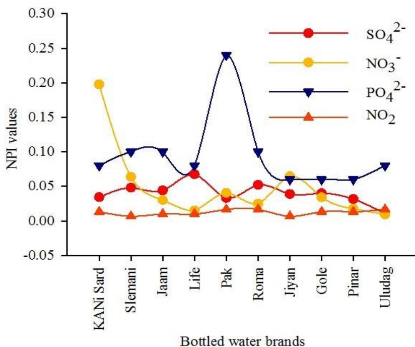
Figure 6: The variation of NPI values of SO 4 2- , NO 3 - , PO 4 2- , and NO 2 .
