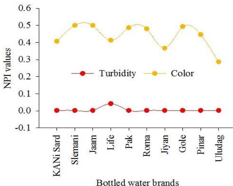
Figure 1: The variation of NPI values of turbidity and color.
