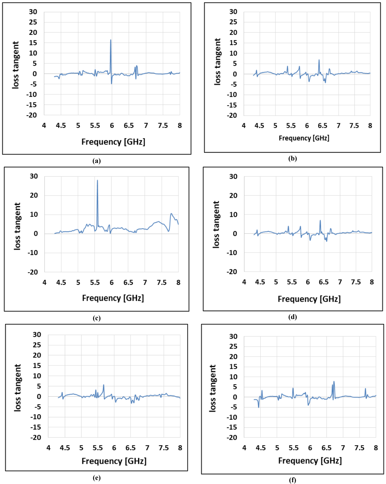
Figure 4: The tangent loss calculated in the C-band frequency for (a) 5% volume fraction Zn_{1-x}Cu_xWO_4(x=0) /epoxy composite (b) 5% volume fraction Zn_{1-x}Cu_xWO_4(x=0.03) /epoxy composite (c) 5% volume fraction Zn_{1-x}Cu_xWO_4(x=0) /polyurethane composite (d) 5% volume fraction Zn_{1-x}Cu_xWO_4(x=0.03) /polyurethane composite (e) 5% volume fraction Zn_{1-x}Cu_xWO_4(x=0) /silicone rubber composite (f) 5% volume fraction Zn_{1-x}Cu_xWO_4(x=0.03) /silicone rubber composite
