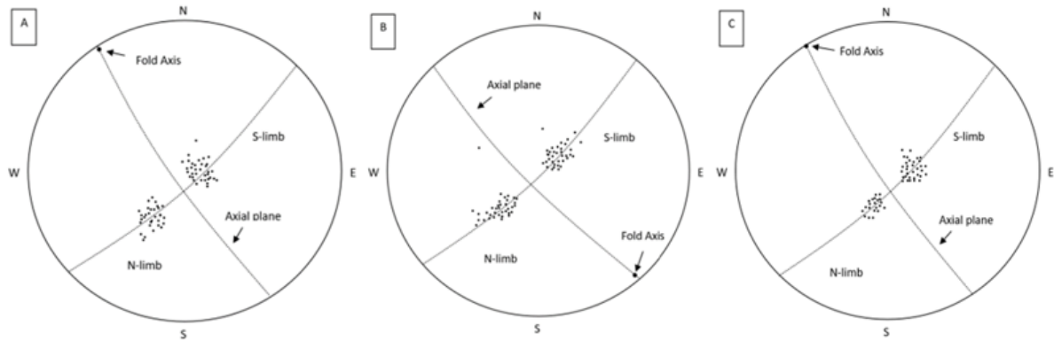
Fig. 10. Shows the stereographic projection of the formations in three traverses.
