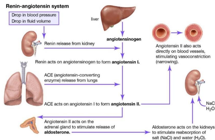
Figure 1. Overview of the Renin-Angiotensin-Aldosterone System (32)
