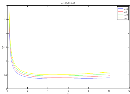
\alpha = 1.5, \beta = 0.2, \theta = 0.5 ve \lambda = 1.5, 2, 2.5, 3 \alpha = 1.5, \theta = 0.2, \lambda = 0.5 ve \beta = 0.9, 1.5, 2, 2.5
