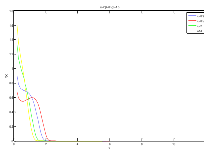
\alpha = 2, \beta = 0.5, \lambda = 0.1 and \theta = 0.2, 0.5, 0.9, 2 \alpha = 2, \beta = 0.5, \theta = 1.5 and \lambda = 0.9, 0.5, 2, 3
