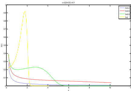
\alpha = 2, \beta = 0.5, \lambda = 0.1 and \theta = 0.2, 0.5, 0.9, 2 \alpha = 2, \beta = 0.5, \theta = 1.5 and \lambda = 0.9, 0.5, 2, 3
