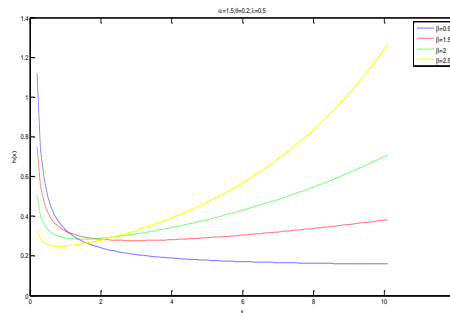
\alpha = 1.5, \beta = 0.2, \theta = 0.5 ve \lambda = 1.5, 2, 2.5, 3 \alpha = 1.5, \theta = 0.2, \lambda = 0.5 ve \beta = 0.9, 1.5, 2, 2.5
