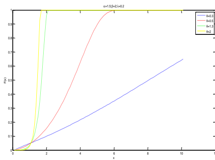
\alpha = 1.5, \beta = 2, \lambda = 0.2 and \theta = 0.3, 0.5, 1.3, 2
