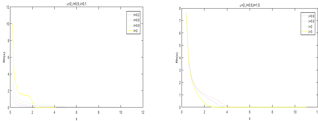
Figure 4. ihf function plots of EP-Ch distribution for different parameter values
