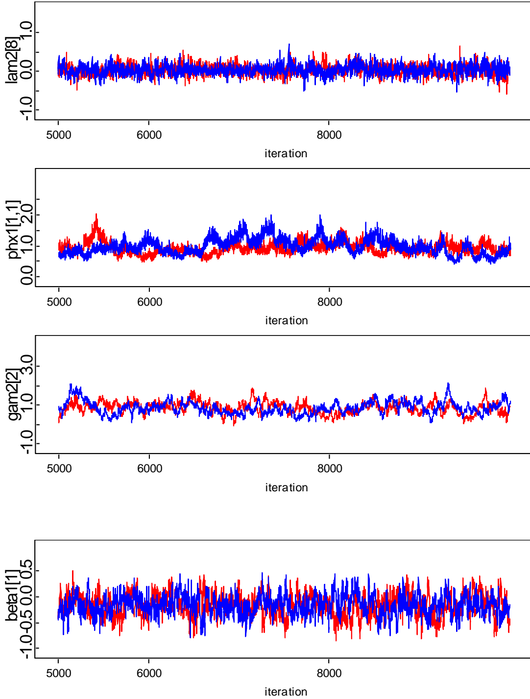
Figure 2. Two chains of observation corresponding to (a) \lambda_8^{(2)} ; (b) \Phi_{11}^{(1)} (c) \gamma_2^{(2)} ; and (d) \beta_1^{(1)} for two populations NLVMs with Dichotomous Variables using Truncated Normal Distribution
