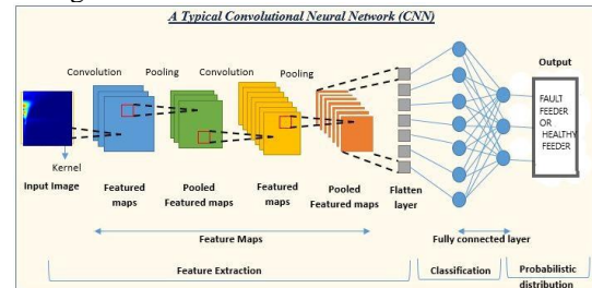
Fig.1 CNN Structure
